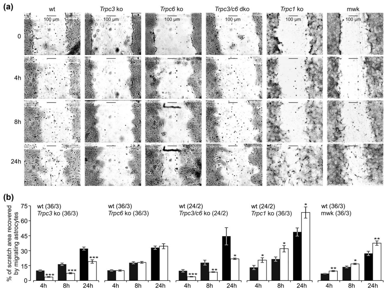
FIGURE 6 In vitro migration of astrocytes depends on Trpc3 and Trpc1 . (a) Representative images of scratched areas in cultured astrocytes isolated from wild-type (wt, black), Trpc3 -/- ( Trpc3 ko, white), Trpc6 -/- ( Trpc6 ko, white), Trpc3 -/- / c6 -/- ( Trpc3/c6 dko, white), Trpc1 -/- ( Trpc1 ko, white) and heterozygous TRPC3 T635A mutant ( mwk , white) mice directly (0 h) and 4, 8 and 24 hours after scratching. (b) Data as in a, plotted as percentage of scratch area recovered by migrating astrocytes 4, 8, and 24 h after scratching. Data in b represent means \pm SEM [n, number of experiments from x, number of cultures (n/x)]. Asterisks assign the significant differences compared to the corresponding wt at the same hour (* p < 0.05 , ** p < 0.01 , *** p < 0.001 )
