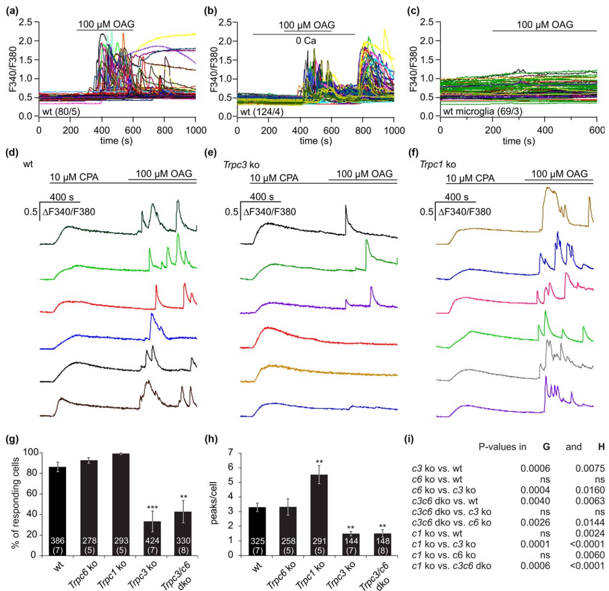
FIGURE 3 OAG-mediated \text{Ca}^{2+} influx depends on TRPC3. (a, b) OAG-induced cytoplasmic \text{Ca}^{2+} increase in astrocytes in the presence (a) and absence of extracellular \text{Ca}^{2+} (b), and upon addition of \text{Ca}^{2+} to the bath as indicated (b). (c) Microglial cells do not reveal a change of cytoplasmic \text{Ca}^{2+} upon OAG application. (d-f) OAG-induced \text{Ca}^{2+} entry in the presence of extracellular \text{Ca}^{2+} (2 mM) at sustained store depletion by cyclopiazonic acid (CPA, 10 \mu\text{M} ) present throughout the experiment in astrocytes from wild-type (wt, d), Trpc3 -/- ( Trpc3 ko, e) and Trpc1 -/- ( Trpc1 ko, f) mice. (g, h) Percentage of OAG-responding cells (g) and number of OAG-mediated \text{Ca}^{2+} peaks per responding cell (h) in astrocytes from wild-type, Trpc6 -/- , Trpc1 -/- , Trpc3 -/- and Trpc3 -/- / c6 -/- mice. Data represent means \pm SEM [n, number of cells from x, number of experiments (n/x)] with asterisks in g and h marking significant differences compared to the wild-type (** p < 0.01 , *** p < 0.001 ). (i) p -values for comparisons in g and h were obtained by one-way ANOVA followed by Bonferroni test [Color figure can be viewed at wileyonlinelibrary.com ]
