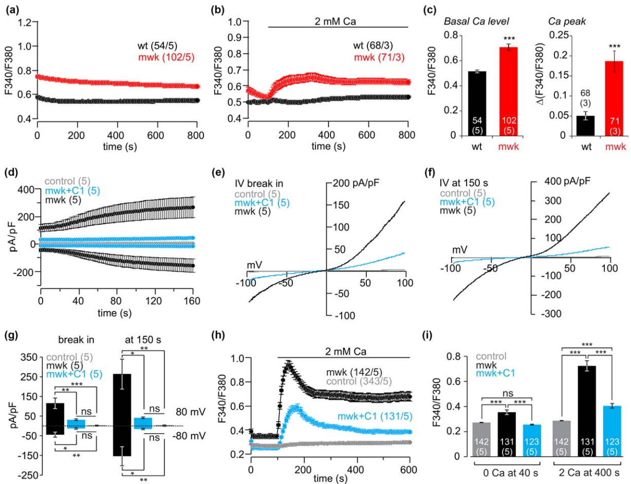
FIGURE 5 Constitutive activity of the TRPC3 T635A moonwalker (mwk) mutant is antagonized by Trpc1 expression. (a, b) Changes of cytoplasmic Ca 2+ (F340/F380) in cultured cortical astrocytes isolated from wild-type (wt) and heterozygous TRPC3 T635A moonwalker (mwk) mice in the presence (a), absence (b, 0–100 s) and after addition (b, application bar) of extracellular Ca 2+ . (c) Basal cytoplasmic Ca 2+ (F340/F380) in a and \Delta F340/F380 upon Ca 2+ readdition in b. (d–g) Spontaneous inward and outward currents at –80 mV and +80 mV in the tetracycline-inducible HEK TRPC3 T635A (mwk) cell line. Control, no tetracycline induction; mwk, after tetracycline induction; mwk + C1, after tetracycline induction and transfection with the Trpc1 cDNA. Current–voltage relationships at break in (e) and at 150 s (f) and corresponding current amplitudes at –80 mV and +80 mV (g), plotted as means \pm SEM (n, number of cells). (h, i) Basal cytoplasmic Ca 2+ and increase of cytoplasmic Ca 2+ upon addition of 2 mM extracellular Ca 2+ . Control, no tetracycline induction; mwk, after tetracycline induction; mwk + C1, after tetracycline induction and transfection with the Trpc1 cDNA. Cytoplasmic Ca 2+ at 40 s and at 400 s (i) plotted as mean \pm SEM [n, number of cells from x, number of experiments (n/x)]. Asterisks assign significant differences (* p < 0.05, ** p < 0.01, *** p < 0.001, ns = not significant) [Color figure can be viewed at wileyonlinelibrary.com ]
