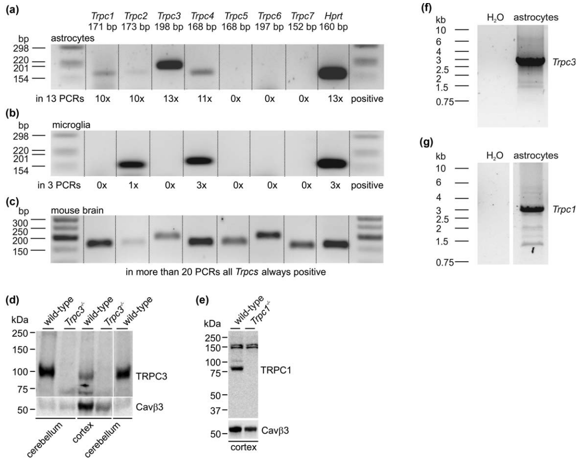
FIGURE 1 Cortical astrocytes express Trpc3 and Trpc1 . (a–c) RT-PCRs performed from 100 FACS-sorted GLAST-positive astrocytes (a), 50 FACS-sorted CD11b-positive microglial cells (b) and mouse brain RNA (c). The frequencies of amplified Trpc transcripts in astrocytes in 13 independent RT-PCRs from 5 independent sortings and in microglia in 3 independent RT-PCRs from 3 independent sortings are shown below the blots. Hprt served as positive control. First and last lanes in a, b and c show marker DNAs. (d, e) Immunoblot analysis of TRPC3 (d) and TRPC1 (e) proteins in lysates from mouse cerebellum and cortex (100 μg/lane) extracted from wild-type and Trpc3 -/- mice or Trpc1 -/- mice revealed the loss of TRPC3 and TRPC1 proteins in Trpc3 -/- and Trpc1 -/- mice, respectively. To confirm equal loading of samples independent blots running in parallel were probed with a Cavβ3 antibody. (f, g) Full-length amplification of Trpc3 (f) and Trpc1 (g) cDNAs from cultured cortical GLAST-positive FACS-sorted astrocytes
