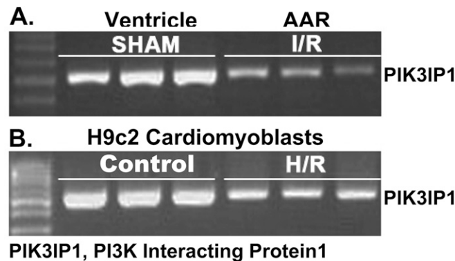
Fig. 54. In vitro H/R treatment of H9c2 cells and in vivo I/R treatment of WT mice reduce the expression of PIK3IP1 to similar extents. Shown are the results from 35-cycle RT-PCR analysis of cardiac RNA (A) and of H9c2 cell RNA (B).
