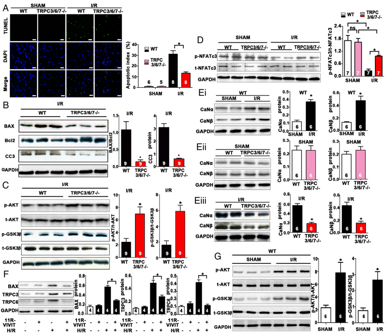
Fig. 5. Injury caused in vivo by I/R involves a positive-feedback loop mediated by NFATc3's transcription of BAX and TRPC genes and is ameliorated by the ablation of TRPC3 and TRPC6 . ( A–E ) Analysis of AARs after I/R showed that, as compared with WT mice, TRPC3/6/7 -/- mice had a decreased proportion of cells undergoing apoptosis ( A ) and, as seen by Western blotting ( B–E ), had decreased levels of the proapoptotic markers BAX and cleaved caspase 3 ( CC3 ) and increased levels of antiapoptotic Bcl2 ( B ); improved levels of survival signaling markers p-AKT and p-GSK3 \beta ( C ); lower levels of activated p-NFATc3 ( D ); and lower levels of Ca \alpha and Ca \beta subunit proteins ( E, i–E, iii ). (Scale bars: 40 \mu m.) ( F ) I/R-activated NFATc3 drives the expression of I/R-induced BAX , TRPC3 , and TRPC6 . ( G ) I/R caused p-AKT and p-GSK3 \beta proteins to increase reflecting activation of the PI3K-signaling pathway. In the Western blot images in all panels, each lane is the blot of an independent cell or mouse tissue sample. Values are means \pm SEM of the indicated number of experiments. * P < 0.05; ns, not significant.
