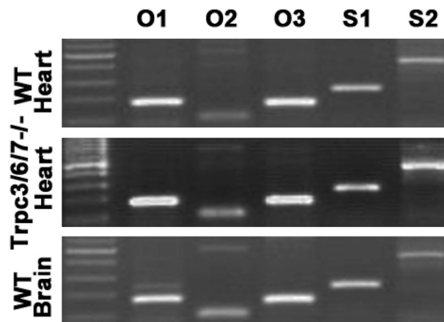
Fig. S2. Cardiac tissues of TRPC3/6/7 -/- and WT mice express similar levels of Orai1, -2, and -3 (O1, O2, and O3) and of STIM1 (S1) and Stim2 (S2) mRNA as seen in 35-cycle RT-PCR.
