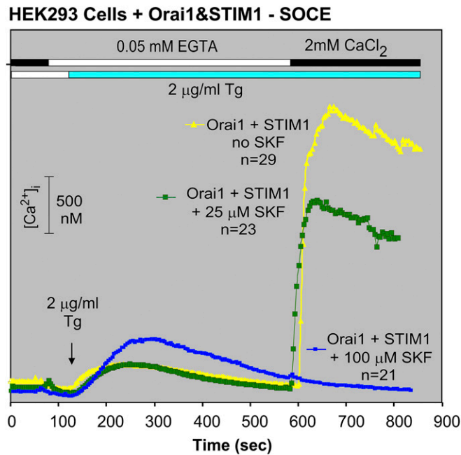
Fig. S1. Although 5 \mu M SKF36365 (SKF) does not affect Orai1-based SOCE (Fig. 1G), higher concentrations do. The figure shows SOCE evoked by thapsigargin (Tg) in HEK293 cells transfected with inhibitory amounts of Orai1 (1 \mu g plasmid per 60-mm dish) and an SOCE-rescuing amount of STIM1 (1 \mu g plasmid per 60-mm dish) in the absence or presence of 25 \mu M or 100 \mu M SKF96365.
