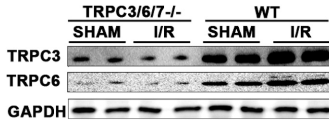
Fig. 53. Long exposure of the Western blot shown in Fig. 3B. The image enhances the relative intensities of the weak bands present at the sites where WT TRPC3 and TRPC6 would be and shows that the weak bands do not change in intensity in same direction as WT bands do in response to I/R ( Discussion ).
