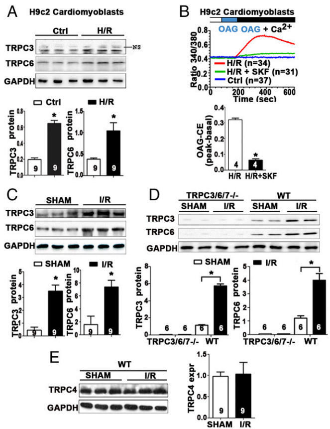
Fig. 3. H/R in vitro and I/R in vivo up-regulate TRPC3 and TRPC6 channel proteins. Each lane is the blot of an independent cell or mouse tissue sample. Bar graphs show summary averages of the indicated number of independent experiments. Data are shown as means \pm SEM; * P < 0.05 for all panels. (A) H/R treatment of H9c2 cardiomyoblasts leads to increased TRPC3 and TRPC6 protein levels. (B) Increased OAG-stimulated Ca ^{2+} entry in response to H/R treatment in H9c2 cardiomyoblasts. The OAG-stimulated Ca ^{2+} entry is inhibited by 5 \mu M SKF96365 (SKF). (C and D) Western blot analyses of TRPC3 and TRPC6 levels in AAR regions of WT and TRPC3/6/7 ^{-/-} hearts from mice subjected to the I/R procedure or in ventricles of sham-operated mice, showing increased TRPC3 and TRPC6 proteins after I/R (C and D) and the absence of TRPC3 and TRPC6 immunoreactivity in the corresponding samples from TRPC3/6/7 ^{-/-} tissues (D), proving antibody specificity. (E) TRPC4 protein levels are unaffected by I/R. Ctrl, control.
