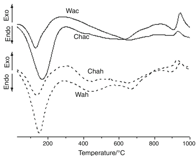
Fig. 2 DTA diagrams of the precursors
