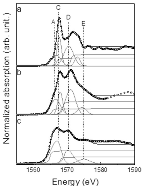
Fig. 6. Al-K XANES spectra of: (a) \alpha -Al 2 O 3 ; (b) Bent-0; and (c) Bent-800. The open circles correspond to the experimental data and full line to fitted results.
