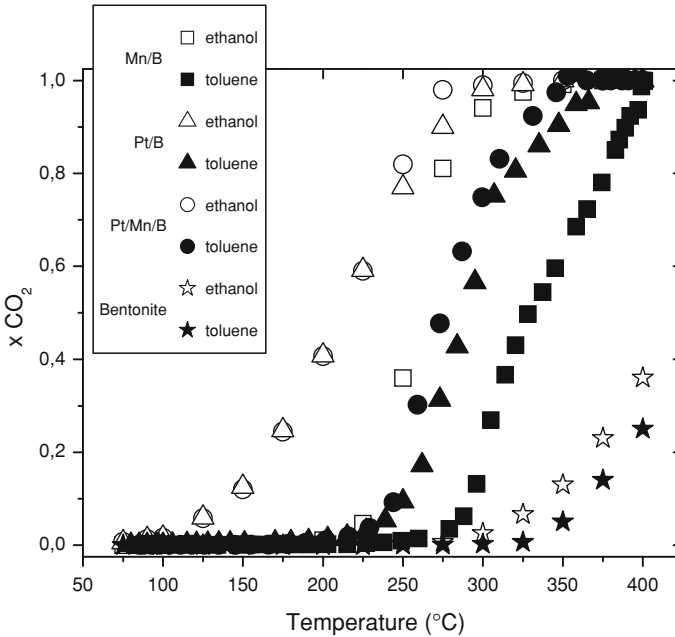
Fig. 5 Ethanol and toluene ignition curves over monoliths
