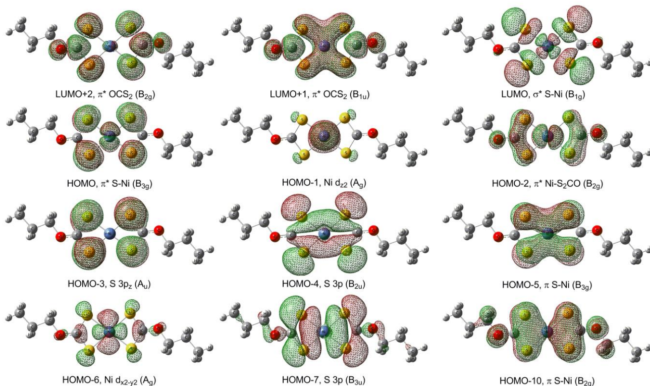
Figure 2. Schematic representation, approximate assignment and symmetry (considering a local D_{2h} symmetry point group) of selected molecular orbitals of \text{Ni}(\text{CH}_3(\text{CH}_2)_2\text{OC}(\text{S})\text{S})_2 , calculated with the TD-B3LYP/6-31+G* approximation.
