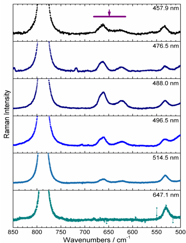
Figure 4. Raman spectra of \text{Ni}(\text{CH}_3(\text{CH}_2)_2\text{OC}(\text{S})\text{S})_2 between 850 and 500 \text{cm}^{-1} excited with wavelengths between 647.1 and 457.9 nm, normalized with respect to the 788 \text{cm}^{-1} band of the solvent (acetone).
