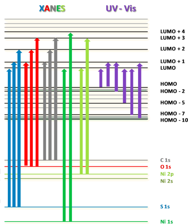
Figure 9. Schematic energy level diagram scheme of Ni(CH 3 (CH 2 ) 2 OC(S)S) 2 showing the electronic transitions extracted from UV-visible and XANES spectra.
