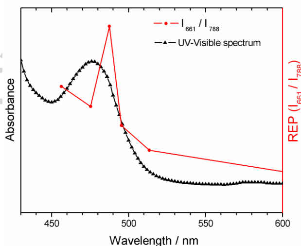
Figure 5. UV-visible spectrum (black trace) and Raman excitation profile of \nu_s(\text{S-C=S}) normalized with respect to the 788 \text{cm}^{-1} Raman band of acetone (red trace) of \text{Ni}(\text{CH}_3(\text{CH}_2)_2\text{OC}(\text{S})\text{S})_2 in acetone solution.
