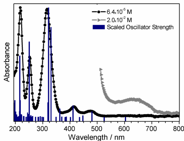
Figure 3. Comparison of the experimental UV-visible spectrum of \text{Ni}(\text{CH}_3(\text{CH}_2)_2\text{OC}(\text{S})\text{S})_2 in \text{CH}_3\text{CN} solution with the scaled one-electron transitions spectrum calculated with the TD-B3LYP/6-31+G* approximation.
