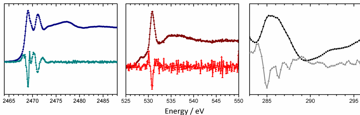
Figure 7. Average of X-ray absorption spectra and second derivative of the spectra of solid \text{Ni}(\text{CH}_3(\text{CH}_2)_2\text{OC}(\text{S})\text{S})_2 measured in the S 1s (left), O 1s (middle) and C 1s (right) energy regions.
