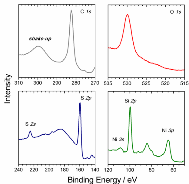
Figure 6. Photoelectron spectra corresponding to the C 1s (310-270 eV, grey), O 1s (535-515 eV, red), S 2s and S 2p (240-150 eV, blue) and Ni 3s and Ni 3p (120-50eV, green) electrons of \text{Ni}(\text{CH}_3(\text{CH}_2)_2\text{OC}(\text{S})\text{S})_2 .
