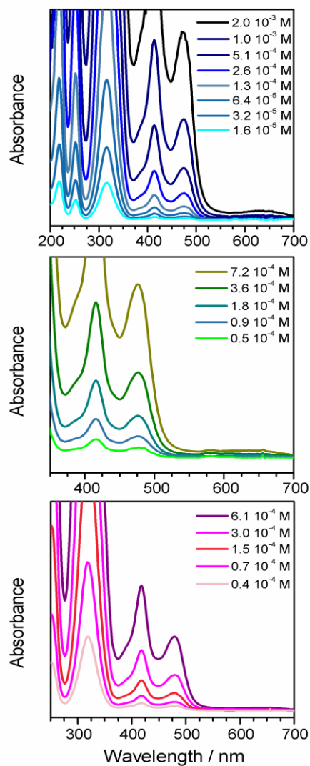
Figure 1. UV-visible spectra of \text{Ni}(\text{CH}_3\text{CH}_2\text{CH}_2\text{OC}(\text{S})\text{S})_2 in solution of \text{CH}_3\text{CN} (top), \text{CH}_3\text{C}(\text{O})\text{CH}_3 (middle) and \text{HCCl}_3 (bottom).
