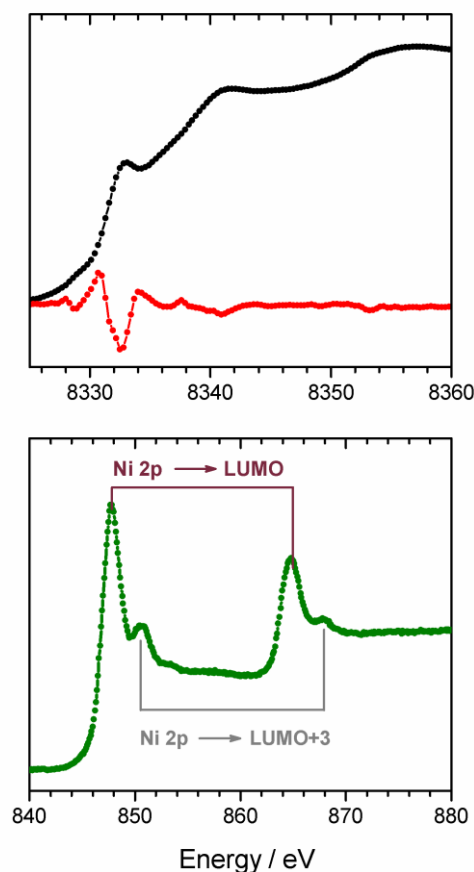
Figure 8. Average of five XANES spectra and second derivative of the spectra of solid \text{Ni}(\text{CH}_3(\text{CH}_2)_2\text{OC}(\text{S})\text{S})_2 measured in the Ni 1s energy region (top) and of ten XANES spectra in the Ni 2p energy region (bottom).
