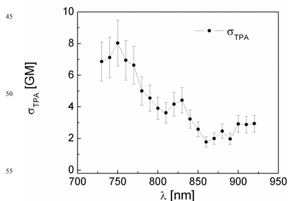
Figure 4. Two-photon absorption spectrum of [Ir(cyclometallated-2-phenylpyridine) 2 (5-Me-1,10-phenanthroline)]PF 6 in CH 2 Cl 2 .
