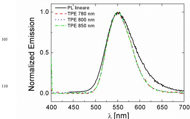
Figure 3. Two-photon emission spectra of cis -[Ir(CO) 2 Cl(4-( para -di- n -butylaminostyryl)pyridine)] in CH 2 Cl 2 excited at various wavelengths.
