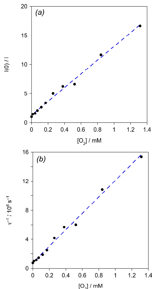
Figure 6. (a) Stern-Volmer plot using the intensity of emission at 565 nm (from spectra shown in Fig. 5) in the absence, I(0) , and presence, I , of oxygen at varying concentrations in oxygen. (b) Plot of the observed decay rate constant ( = reciprocal of luminescence lifetime) as a function of [O_2] . The blue dashed lines show the least-squares linear fit to the data.
