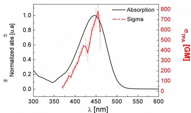
Figure 2. One-photon absorption (black full line) and two-photon absorption (red line + symbol) spectra of cis -[Ir(CO) 2 Cl(4-( para -di- n -butylaminostyryl)pyridine)] in CH 2 Cl 2 . The abscissa scale of the TPA spectrum is divided by two to have a direct comparison with the OPA spectrum.
