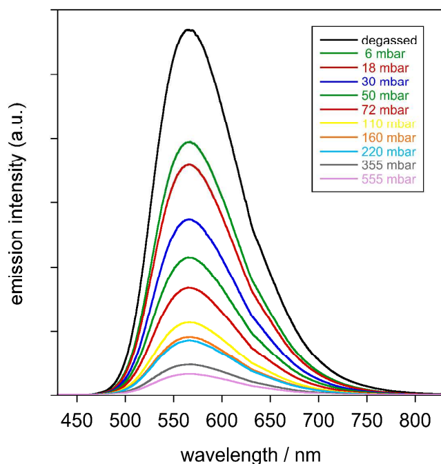
Figure 5. Emission spectra of complex 2 in CHCl_3 at 298 K, recorded in degassed solution ( p < 10^{-2} mbar) (black line) and at variable pressures of air as indicated in the inset. \lambda_{ex} = 400 nm.
