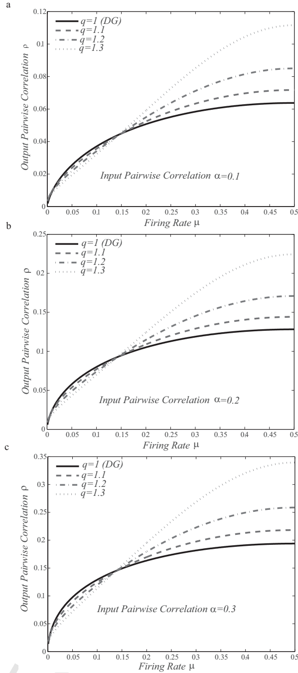
Fig. 5. Output correlation \rho as function of the firing rate \mu , taking q = 1 , q = 1.1 , q = 1.2 and q = 1.3 . (a) Considering a fixed input correlation \alpha = 0.1 . (b) Input correlation \alpha = 0.2 . (c) Input correlation \alpha = 0.3 .
