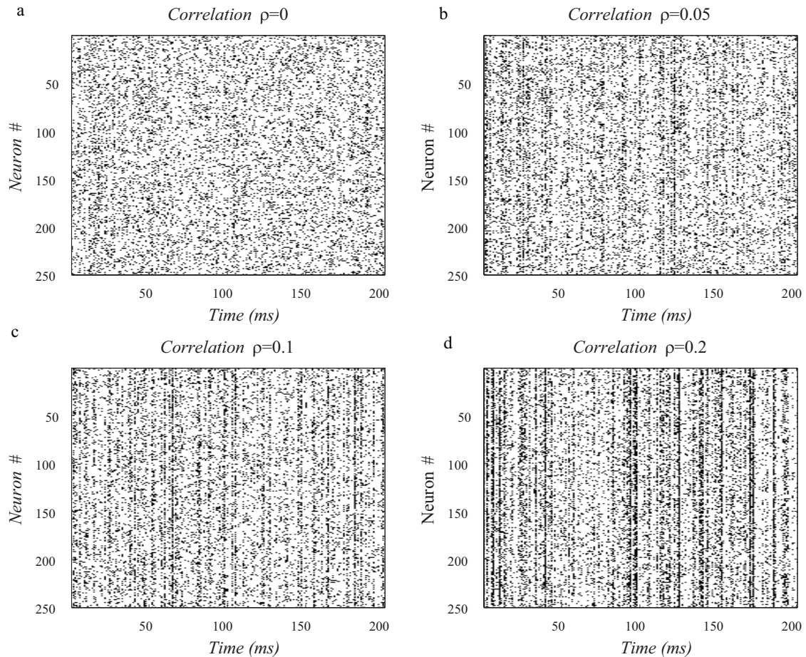
Fig. 2. Same as in Figure 1 but considering q-DG formalism with q = 1.35 . (a) \rho = 0 , (b) \rho = 0.05 , (c) \rho = 0.1 and (d) \rho = 0.2 . Note that in comparison with Figure 1, higher values of spike synchronization are visible at simple sight due to the larger amount of input correlation.
