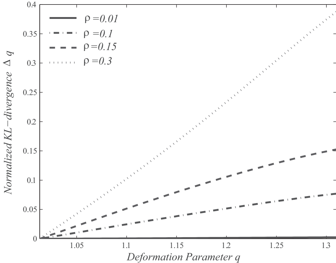
Fig. 7. The normalized Kullback-Leibler divergence versus the deformation parameter q , given different output correlation values \rho = 0.01 , \rho = 0.1 , \rho = 0.15 and \rho = 0.3 (the reference distribution is taken as \rho = 0 for each value of \rho , and it is normalized to the distribution with q = 1 as in Eq.(29)).
