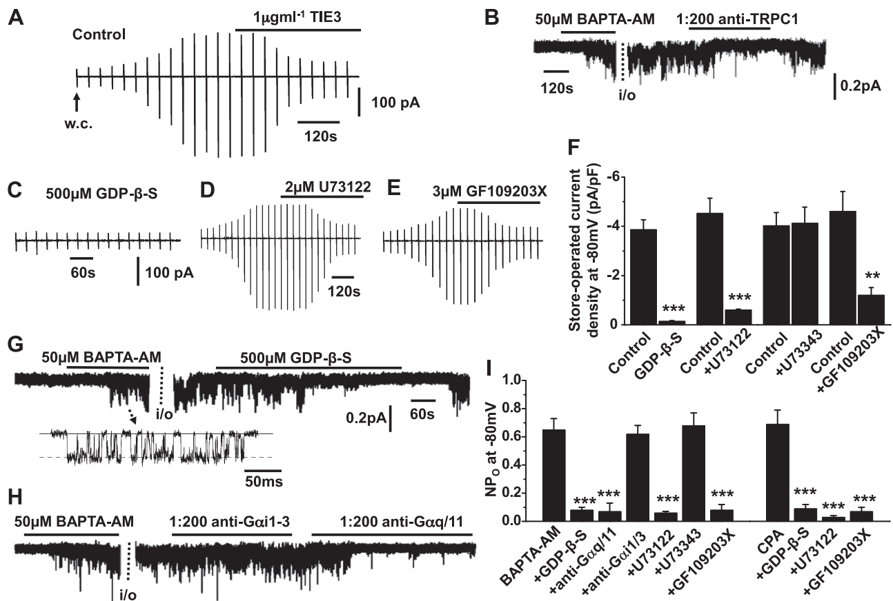
Figure 1. G-proteins, PLC, and PKC activities mediate TRPC1 SOCs. A ) Representative recording shows development of a store-operated whole-cell cation current following break-in into the whole-cell configuration (w.c.), which was inhibited by bath application of the external-acting TRPC1 antibody TIE3. Vertical deflections represent currents evoked by voltage ramps from +100 to -150 mV (750 ms duration) every 30 s from a holding potential of 0 mV. B ) Representative trace shows that BAPTA-AM-evoked single cation channel activity in cell-attached patches held at -80 mV was maintained following patch excision into the inside out configuration (i/o) and inhibited by bath application of an internal-acting TRPC1. C ) Trace shows that development of a store-operated whole-cell TRPC1 current was prevented by inclusion of GDP-β-S in the patch pipette solution. D, E ) Store-operated whole-cell TRPC1 currents were inhibited by bath applications of U731222 or GF109203X, respectively. F ) Mean data show the inhibitory effects of GDP-β-S, U73122, and GF109203X on store-operated whole-cell TRPC1 current densities at -80 mV (each data set is n = 6 ). *** P < 0.001 . G, H ) Original recording traces show that BAPTA-AM-evoked single cation channel activity in cell-attached patches held at -80 mV was inhibited by GDP-β-S or a mixture of anti-Gαq and anti-Gα11 antibodies to the cytosolic surface of inside out patches, whereas a mixture of anti-Gαi1/2 and anti-Gαi3 antibodies had no effect. I ) Mean data show inhibitory actions of GDP-β-S, anti-Gαq/11 antibodies, U73122, and GF109203X on BAPTA-AM-evoked TRPC1 channel activity (each data set is n = 6 ). ** P < 0.01 ; *** P < 0.001 .
