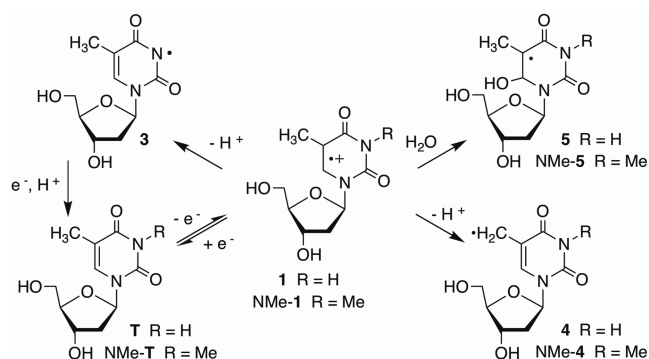
Scheme 1. Formation and Reactivity of the Thymidine Radical Cation
