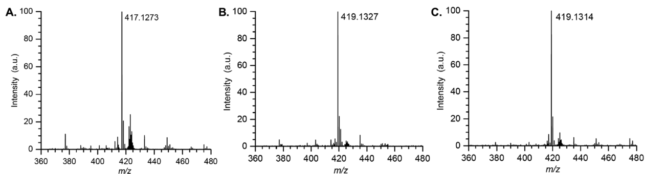
Figure 3. ESI-MS spectra of obtained NMe-14 from photolysis of NMe-6 in the presence of (A) \text{H}_2\text{O}/\text{O}_2 , (B) \text{H}_2^{18}\text{O}/\text{O}_2 , and \text{H}_2\text{O}/^{18}\text{O}_2 .
