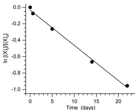
Figure 1. Decomposition of desilylated 11 ( X ) in CD 3 OD/phosphate buffered saline ( v/v = 1:1) monitored by 31 P NMR.
