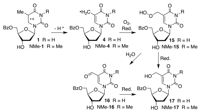
Scheme 5. Anticipated Products following C5-Deprotonation from the Radical Cation
