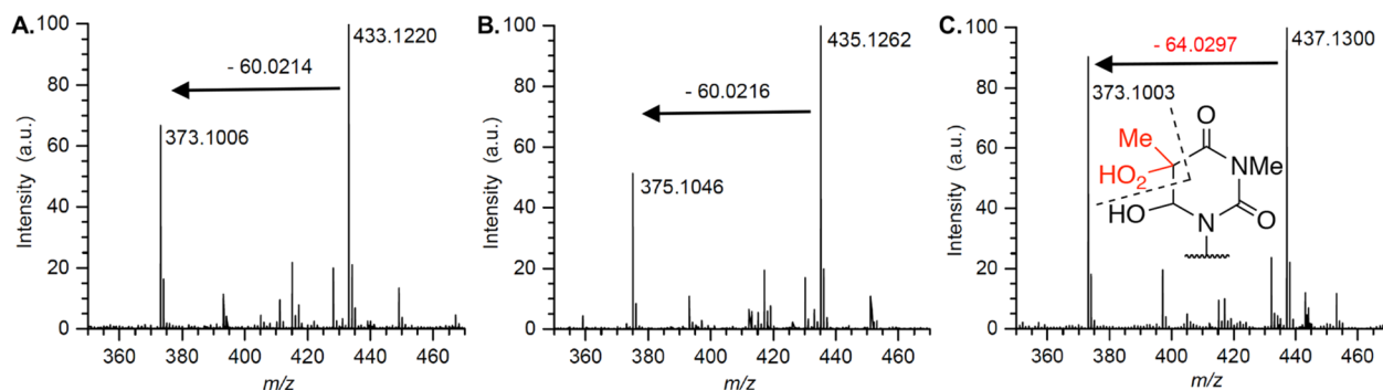
Figure 2. ESI-MS spectra of obtained NMe-13 from photolysis of NMe-6 in the presence of (A) \text{H}_2\text{O}/\text{O}_2 , (B) \text{H}_2^{18}\text{O}/\text{O}_2 , and \text{H}_2\text{O}/^{18}\text{O}_2 .
