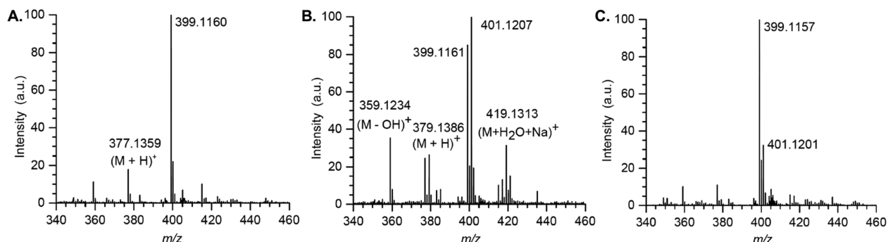
Figure 4. ESI-MS spectra of NMe-17 from photolysis of NMe-6 in the presence of \text{H}_2\text{O}/\text{H}_2^{18}\text{O} and \text{O}_2/^{18}\text{O}_2 .
