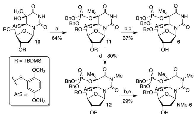
Scheme 3. Syntheses of Radical Cation Precursors a
