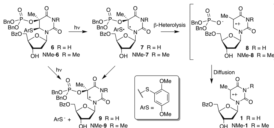
Scheme 2. Photochemical Radical Cation Generation
