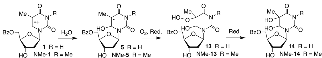
Scheme 4. Anticipated Products following Radical Cation Hydration
