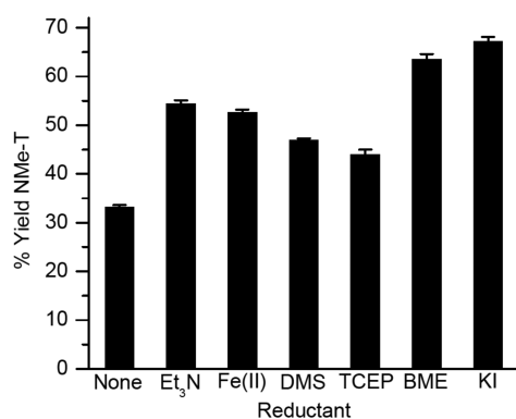
Figure 5. Effect of reductant (10 mM) on the yield of NMe-T from photolysis of NMe-6. DMS = dimethyl sulfide. TCEP = tris-(carboxyethyl)phosphine.
