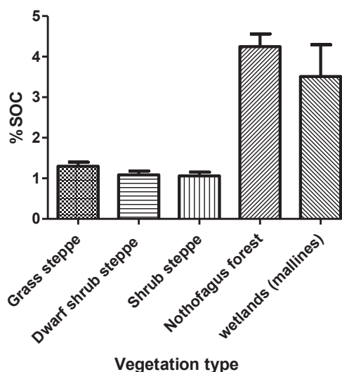
Fig. 2. Soil carbon concentration (%SOC) across vegetation types in Santa Cruz Province, Southern Patagonia.
