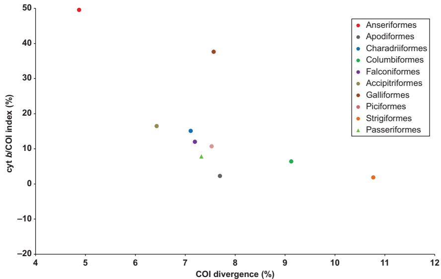
Figure 3. Association between the mean difference in divergence between cyt b and COI ( cyt b /COI index) and the mean COI uncorrected p-distance for ten avian orders. Pearson correlation coefficient ( r = -0.72 , p < 0.001 ). The correlation was performed after weighting the mean index values of each order by the number of pair of species compared within each of them. Positive index values indicate higher divergence in cyt b than in COI.
