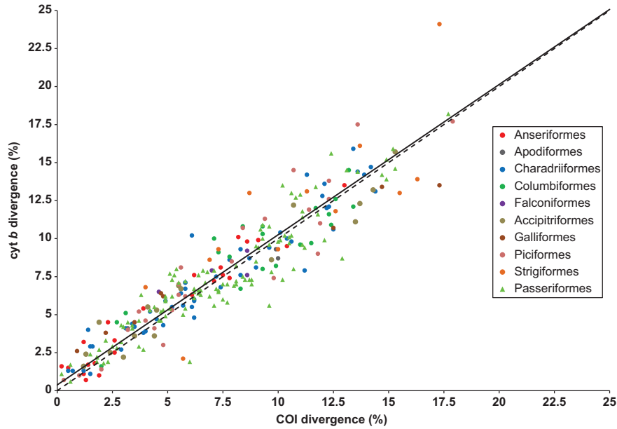
Figure 1. Comparison of uncorrected p-distances for COI and cyt b in 278 phylogenetically independent pairs of species. The dashed line shows equal divergence between the two loci. The solid line corresponds to the reduced major axis regression ( \text{cyt } b = 0.9879 \times \text{COI} + 0.3774 , r^2 = 0.87 , where cyt b and COI correspond to genetic distances in each gene). Pearson correlation coefficient ( r = 0.93 , p < 0.0001 ). Shape and colour of the symbols indicate the order to which each pair of species belongs.
