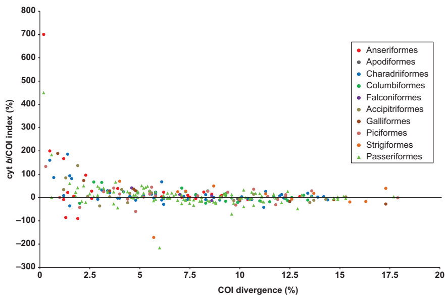
Figure 2. Decay of the difference in divergence between cyt b and COI ( cyt b /COI index) as the uncorrected p-distance for COI between the species being compared increases. Positive index values indicate higher divergence in cyt b than in COI, whereas negative values are the reverse. Shape and colour of the symbols indicate the order to which each pair of species belongs.
