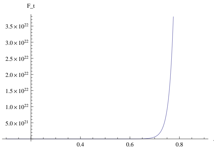
Figure 1: The black hole self force function of s = 1 - r^{-2} , from s = 0 to s = 0.9 to order n = 25 . The force seems to grow, but the next figure shows that it attach a maximum.
