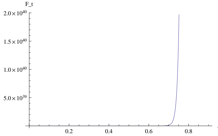
Figure 3: The force for n = 45 in the interval from s = 0 to s = 0.9 .
