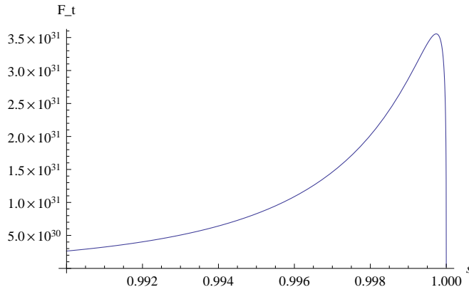
Figure 2: The behavior of the self force near the boundary s = 1 . It reaches a maximum and then goes to zero. We argue that this is just an effect of the truncation of the series and that the line s = 1 is in fact an asymptote.
