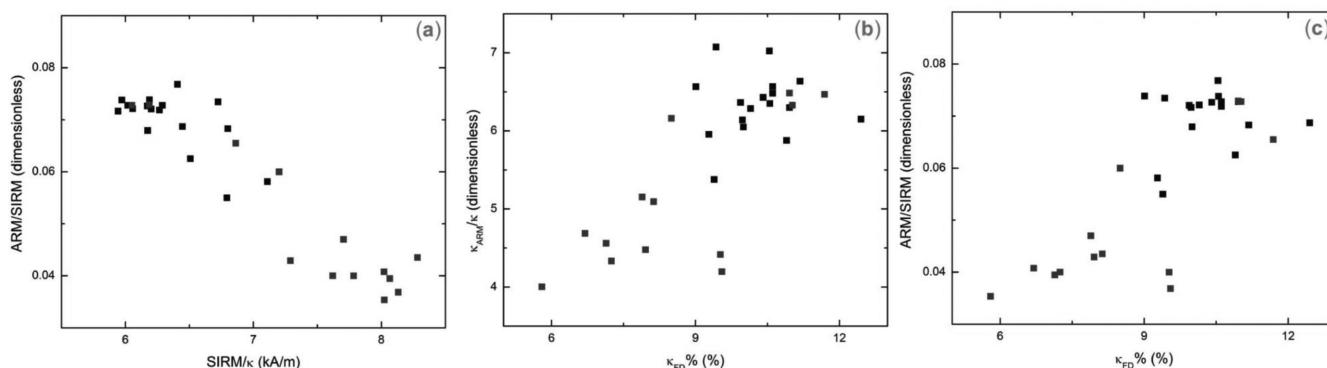
Figure 11. Biplot of (a) ARM/SIRM versus SIRM/ \kappa , (b) \kappa_{\text{ARM}}/\kappa versus \kappa_{\text{FD}}\% and (c) ARM/SIRM versus \kappa_{\text{FD}}\% for selected samples.
