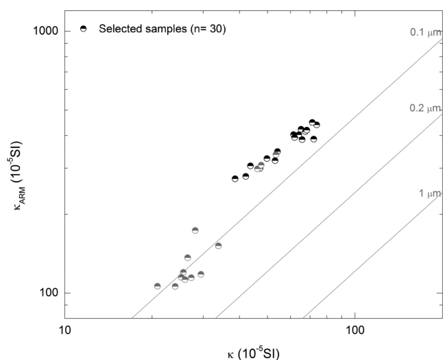
Figure 10. King's plot ( \kappa_{ARM} versus \kappa ) for selected samples. Two grouping are observed: samples at 30 cm (upper part) and at 50 cm (lower part, in grey colour).
