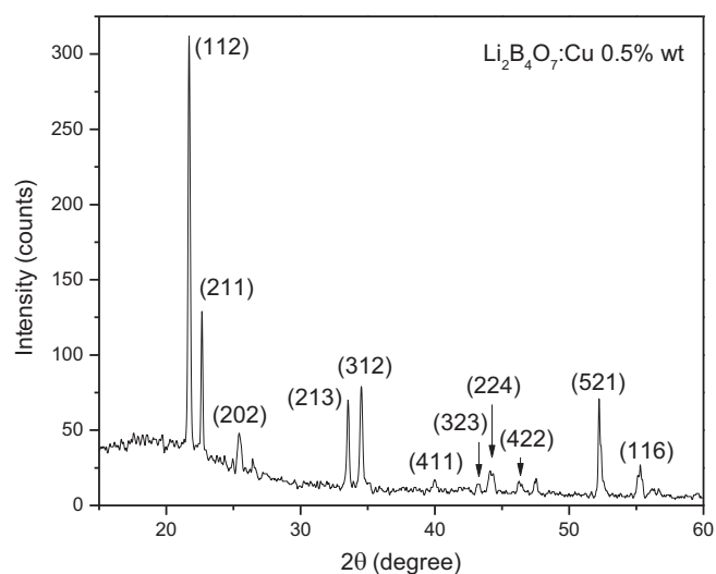
FIGURE 1. X-ray diffraction pattern of Li 2 B 4 O 7 :Cu
