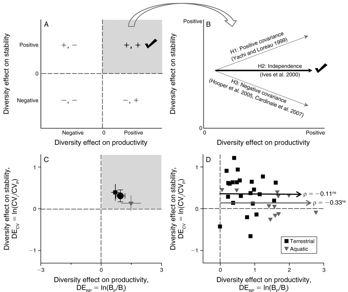
FIG. 1. Effects of biodiversity on the productivity and stability of biomass. In this study we addressed two distinct questions: (A) What is the joint distribution of data describing how biodiversity impacts both the production of biomass, and the stability of biomass through time? (B) How do diversity effects on production covary with the effects of diversity on stability (see Introduction for three contrasting predictions)? Check marks signify which hypotheses were supported. Our re-analysis of 34 biodiversity experiments performed with plants and algae shows that (C) producer species richness simultaneously enhances both the production of biomass ( x -axis) and the stability of biomass through time ( y -axis; see Table 1 for a description of metrics). Data points give the mean effect sizes \pm 95\% confidence intervals for terrestrial (square) and aquatic (triangle) studies, and collectively for all 34 experiments (black circle). Note that studies generally fall within quadrant 1, corresponding to the upper right of panel A. Our re-analysis also shows that (D) diversity effects on biomass production are independent of diversity effects on temporal stability. Each data point gives results for one experiment ( N = 23 terrestrial, 11 aquatic). Spearman rank correlations ( \rho ) illustrate the covariance between the magnitude of the two diversity effects (i.e., correlation between x and y data points); "ns" indicates not significant.
