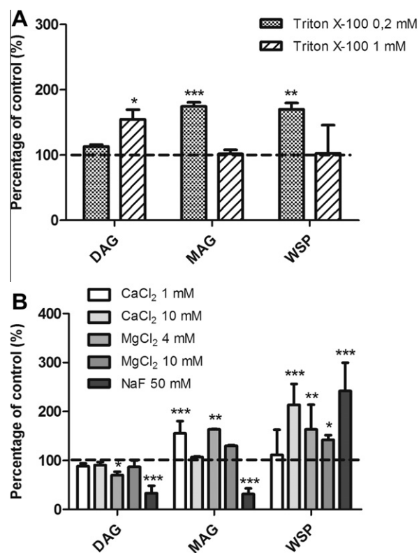
Fig. 5. Effects of detergents and ions on DAG and MAG production in isolated nuclei of rat liver. DAG and MAG production was determined in the presence of the non-ionic detergent Triton X-100 (A) and in the presence of Ca 2+ , Mg 2+ or NaF (B). All assays were conducted under the same conditions as described in Fig. 2. Results are indicated as a percentage of control values (controls represent 100%) and they represent the mean ± S.D. of three individual samples. * P < 0.05, ** P < 0.005, *** P < 0.0005 with respect to control values.
