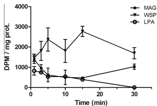
Fig. 6. PA-PLA activity in isolated nuclei of rat liver. MAG, WSP and LPA were determined incubating 40 μg of nuclear protein and 0.2 mM of [ 3 H]PA as a substrate in the corresponding assay buffer, as function of time. Results represent the mean ± S.D. of three individual samples.
