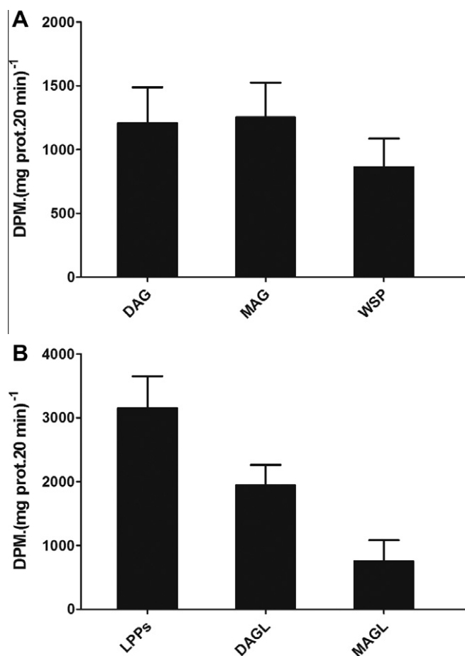
Fig. 2. Metabolism of [ 3 H]-PA in isolated nuclei of rat liver. LPPs, DAGL and MAGL activities were determined using 80 μM [ 3 H]PA and 40 μg of nuclear protein in a final volume of 100 μl, as was described in Section 2.5.1. DAGL activity was determined by monitoring the formation rate of monoacyl[2- 3 H]glycerol using, as substrate, diacyl[2- 3 H]glycerol derived from LPP action on [ 3 H]PA. MAGL activity was determined by monitoring the formation rate of [2- 3 H]glycerol-WSP using monoacyl[2- 3 H]glycerol derived from diacyl[2- 3 H]glycerol. The subsequent procedure is specified in Section 2. In (A) and (B) results represent the mean ± S.D. of 11 individual samples.
