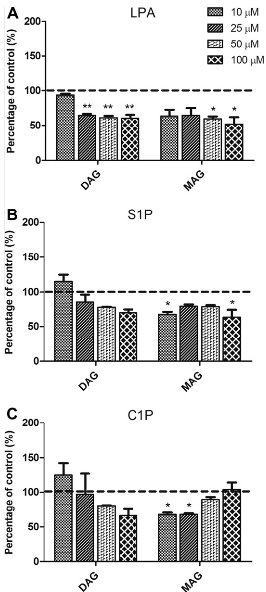
Fig. 4. Metabolism of [ 3 H]PA in the presence of LPA, S1P and C1P in isolated nuclei of rat liver. The effects of LPA (A), S1P (B) and C1P (C) on PA hydrolysis were evaluated using 80 μM [ 3 H]PA in the presence of LPA, S1P or C1P at the indicated concentrations. The subsequent procedure is specified in Section 2. Results represent the mean ± S.D. of three individual samples. * P < 0.05, ** P < 0.005 with respect to the absence of LPA, S1P or C1P.
