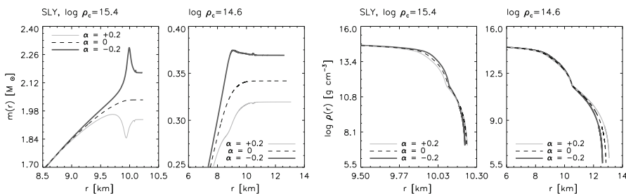
Fig. 3 Zoom-in of the the mass and density profiles close of the surface of the NS for the SLY EoS shown in Fig. 2, for \rho_c = 10^{15.4} and 10^{14.6} \text{ gr cm}^{-3} . For the value of the \alpha parameter -0.2 \text{ km}^2 ( +0.2 \text{ km}^2 ) the mass increases (decreases) roughly 10% respect to de GR case ( \alpha = 0 ), for both low and high central densities
