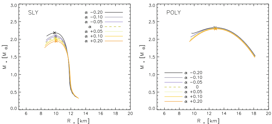
Fig. 1 Mass-radius ( M_\star - R_\star ) relations for the two selected EoS: SLY and POLY (left and right, respectively), considering seven values for the \alpha parameter, which are indicated above in \text{km}^2 units. All the curves correspond to values of central density, \rho_c , in the range 10^{14.6} - 10^{15.9} \text{ gr cm}^{-3} . The crosses indicate the maximum mass for each curve, assuming a necessary condition for equilibrium: dM/d\rho_c > 0
