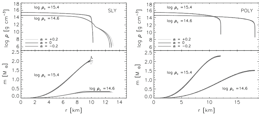
Fig. 2 Profiles of the internal structure of NSs for two extreme cases of low and high central densities, \rho_c = 10^{14.6} and 10^{15.4} \text{ gr cm}^{-3} , and for three different values of the \alpha parameter ( +0.2, 0.0 and -0.2 \text{ km}^2 ), where \alpha = 0.0 corresponds to GR case. On the left ( right ) panel profiles corresponding to the SLY (POLY) EoS are shown. A zoom-in of the mass profile close to the NS surface is shown in Fig. 3. At low central density values the effect on the integrated mass can still represent a deviation as much as \leq 10\% from the GR mass
