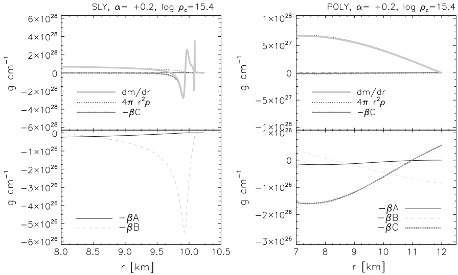
Fig. 5 Profile of the mass gradient, dm/dr (thick line), close to the surface of the NSs for SLY (left panel) and POLY (right panel) EoSs. Deviations of the mass profile from the GR case are much more important for the realistic SLY EoS. Note that the dashed line indicates zeroth-order (GR) term and the continuous with plus signs line indicates the contribution of the C \propto R_0''/R_0 term. Lower panels zoomed-in to show in detail the contribution of the minor perturbative terms, indicated in the legend
