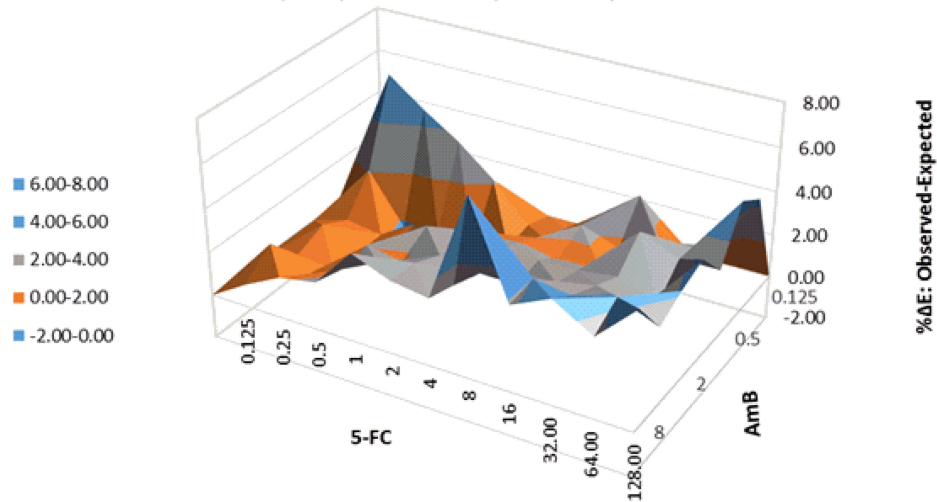
Bliss independence 3-dimensional plot: Rhinocladiella mackenziei (CBS 109634)
