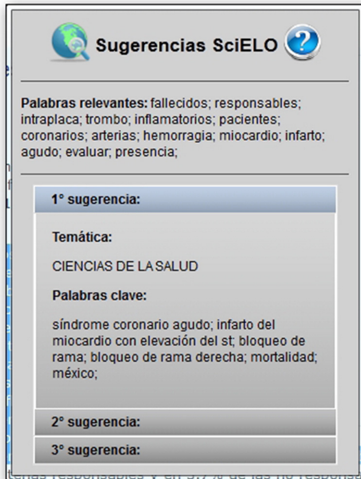
Fig. 3. The SciELO Suggester's interface showing the relevant terms and generated suggestions, including the subject areas and their associated keywords.
