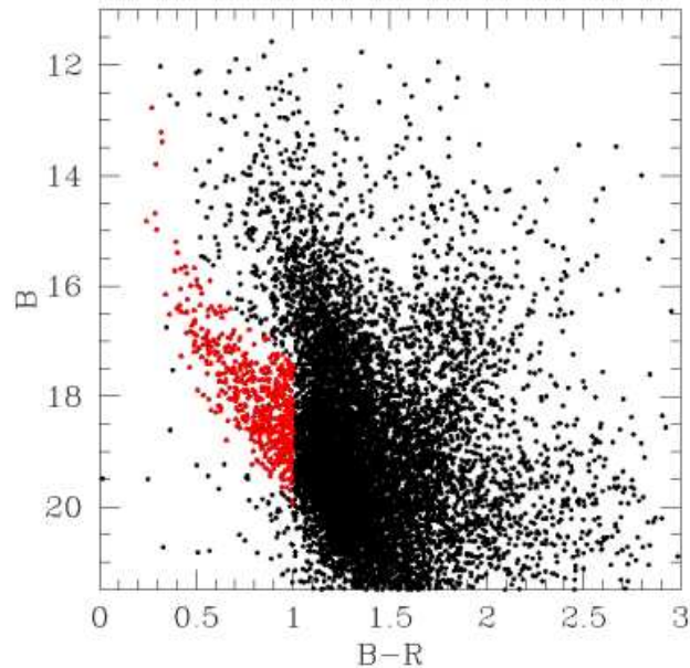
Figure 5. The CMD in the B-R vs B plane of all stars having photometric errors smaller than 0.1 in the direction of the CMa over-density
