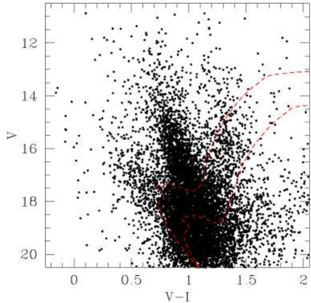
Figure 12. V vs V-I CMD of the CMa over-density. Two isochrones (dashed lines, red when printed in color) have been superimposed to guide the eye, illustrate the position of the TO, and provide a rough estimate of the mean age of the population.
