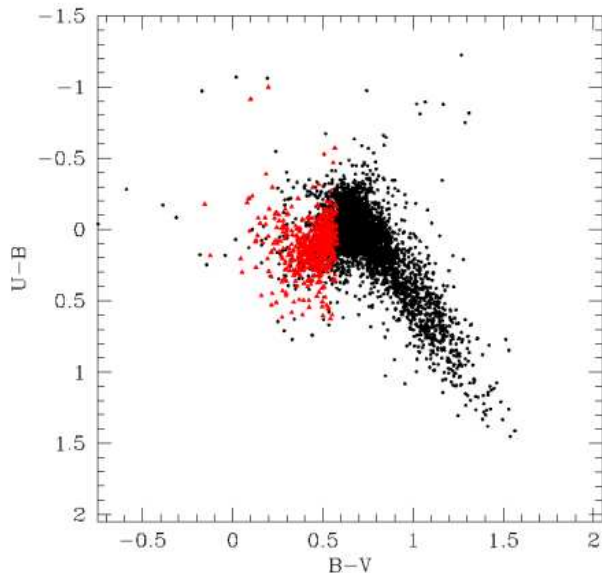
Figure 9. TCD for all the stars having photometric errors smaller than 0.1 mag in the direction of the CMa over-density. With filled triangles (red when printed in color) we indicate stars belonging to the blue plumes , as selected in the B-R vs B CMD.
