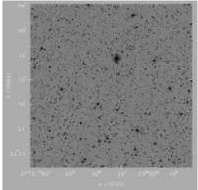
Figure 3. 20 arcmin on a side field in the CMa over-density (Field 3). This field is centered at RA = 07:20:21, DEC = -31:15:43. North is up, East to the left.
