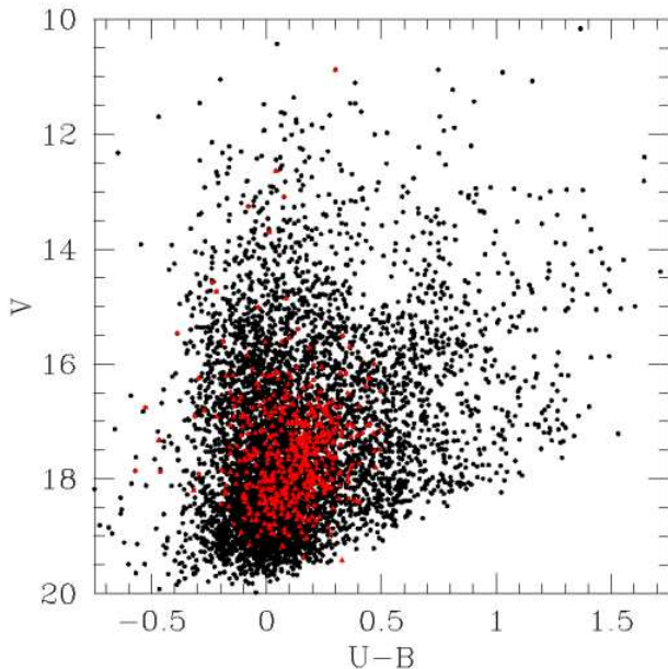
Figure 8. The CMD in the U-B vs V plane of all stars having photometric errors smaller than 0.1 in the direction of the CMA over-density. With filled triangles (red when printed in color) we indicate stars belonging to the blue plumes , as selected in the B-R vs B CMD.
