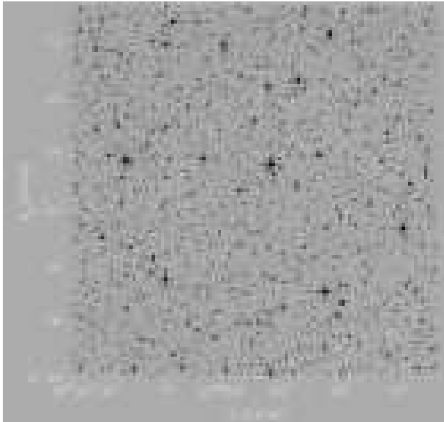
Figure 1. 20 arcmin on a side field in the CMa over-density (Field 1). This field is centered at RA = 07:22:51, DEC = -30:59:20. North is up, East to the left
