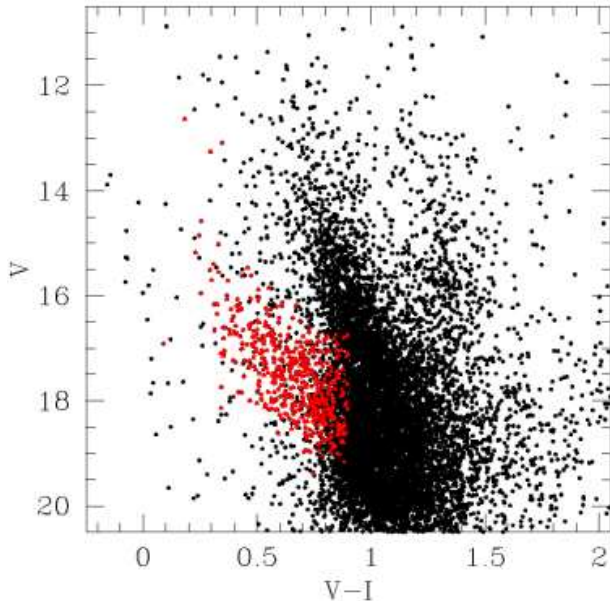
Figure 7. The CMD in the V-I vs V plane of all stars having photometric errors smaller than 0.1 in the direction of the CMA over-density. With filled triangles (red when printed in color) we indicate stars belonging to the blue plumes , as selected in the B-R vs B CMD.
