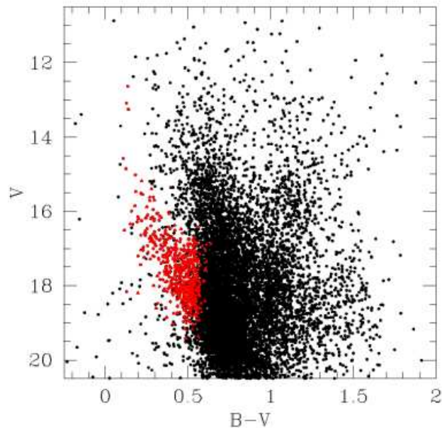
Figure 6. The CMD in the B-V vs V plane of all stars having photometric errors smaller than 0.1 in the direction of the CMa over-density. With filled triangles (red when printed in color) we indicate stars belonging to the blue plumes , as selected in the B-R vs B CMD.
