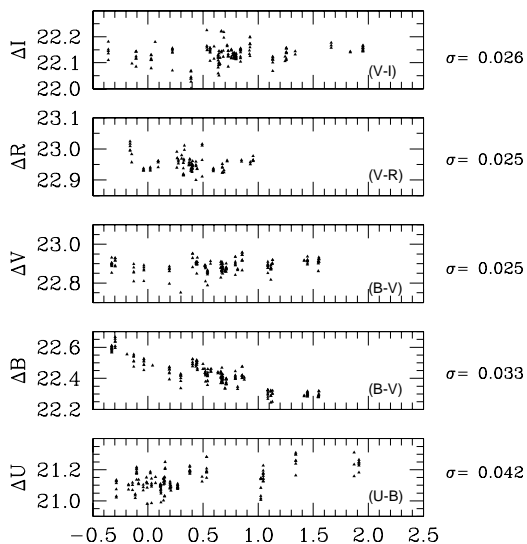
Figure 4. Photometric solution in UBVR for standard stars. See Table 2 for details. \sigma , on the right, indicates the rms of the fit.
