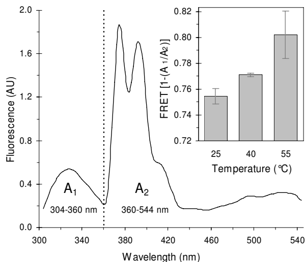
Figure 4 Förster resonance energy transfer (FRET) from the AChR. Smoothened fluorescence emission spectrum of an AChR PyPC-containing sample at 25 °C showing the areas ( A_1 and A_2 ) used to evaluate FRET. The dotted line indicates the average boundary wavelength at which the absolute value of the first derivative of the spectrum passed through a minimum. Excitation wavelength = 290 nm. Inset: FRET from AChR to PyPC as a function of temperature. FRET was calculated according to [1 - (A_1/A_2)] . Liposomes contained DOPA/DOPC/NBD-Chol at a molar fraction 20/40/40 and a lipid to protein molar ratio of 500:1. PyPC concentration was 5 mol%. Error bars represent the S.D. of two independent samples.
