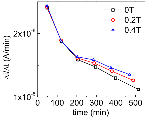
FIG. 3. Time dependence of the transient photocurrent rate for ZOH film, at different applied magnetic fields at 305 K.
