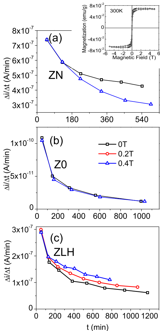
FIG. 2. Variation of the transient photocurrent rate at different applied magnetic fields, as a function of the total time for the thin film samples (a) ZN and (b) ZO and the single microwire (c) ZLH. All measurements were done at a fixed temperature of 305 K. The inset in (a) shows the field loop of the magnetization measured for the ZN film at 300 K.
