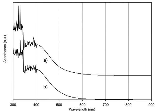
Figure 2. UV/Vis spectra of: a) commercial Wilkinson complex and b) regenerated Wilkinson complex
