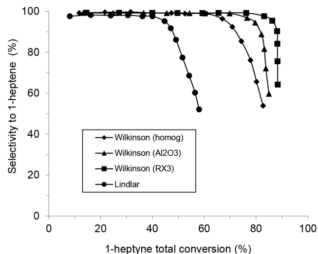
Figure 5. Selectivity to 1-heptene as a function of 1-heptyne total conversion, for the commercial Wilkinson complex in homogeneous and heterogeneous systems, and for the Lindlar catalyst
