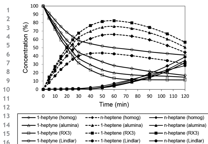
Figure 3. Concentration profiles of reactants and products as a function of time for the commercial Wilkinson complex in homogeneous and heterogeneous systems, and for the Lindlar catalyst
