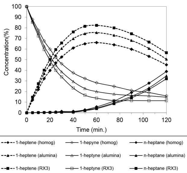
Figure 6. Concentration profiles of reactants and products as a function of time for the regenerated Wilkinson complex in homogeneous and heterogeneous systems
