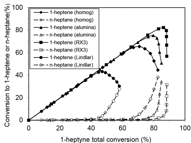
Figure 4. Conversion of 1-heptyne to 1-heptene (solid lines) and conversion of 1-heptyne to n-heptane (dashed lines) as a function of 1-heptyne total conversion, for the commercial Wilkinson complex in homogeneous and heterogeneous systems, and for the Lindlar catalyst
