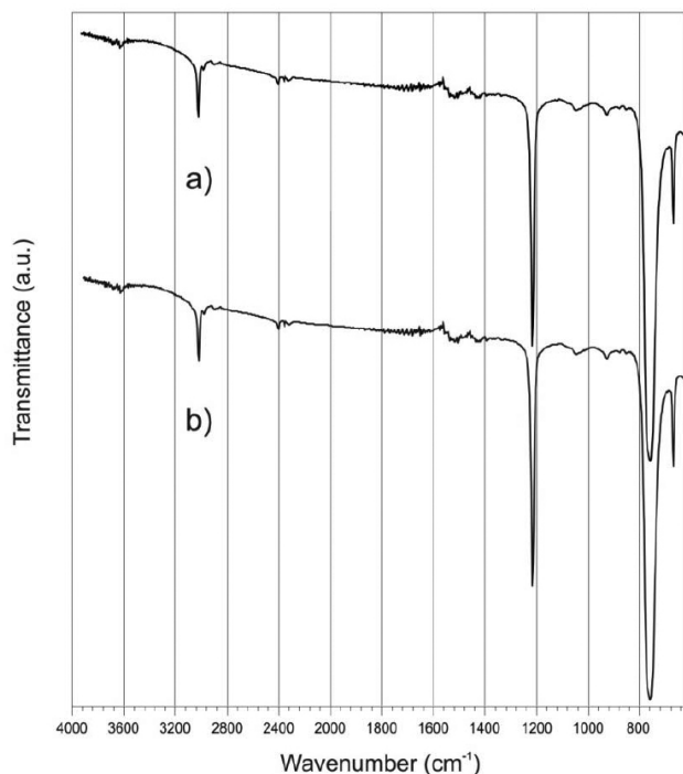
Figure 1. FTIR spectra of: a) commercial Wilkinson complex and b) regenerated Wilkinson complex
