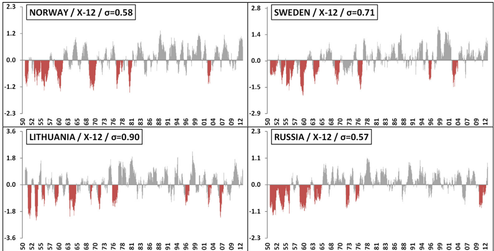
Fig. 4. Northern Europe country drought series for the period 1950–2012 according to the indicator X-12 for some selected countries. Drought events are marked in red.
