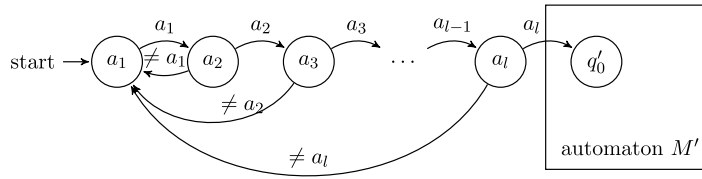
Fig. 1. The automaton M . \rho = a_1 \dots a_l is a synchronizing word, and M' “translates” \hat{M} , which has inputs on the language of edges, \mathcal{E}(G)^* to the language L(X) \subseteq \Sigma^* .
