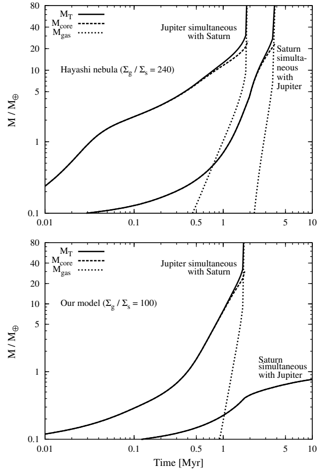
Fig. 17. Comparison of the simultaneous formation of Jupiter and Saturn for a 6 MMSN disk for the Hayashi nebula ( \Sigma_g/\Sigma_s = 240 ) and our model ( \Sigma_g/\Sigma_s = 100 ). The formation processes are very different in each case.
