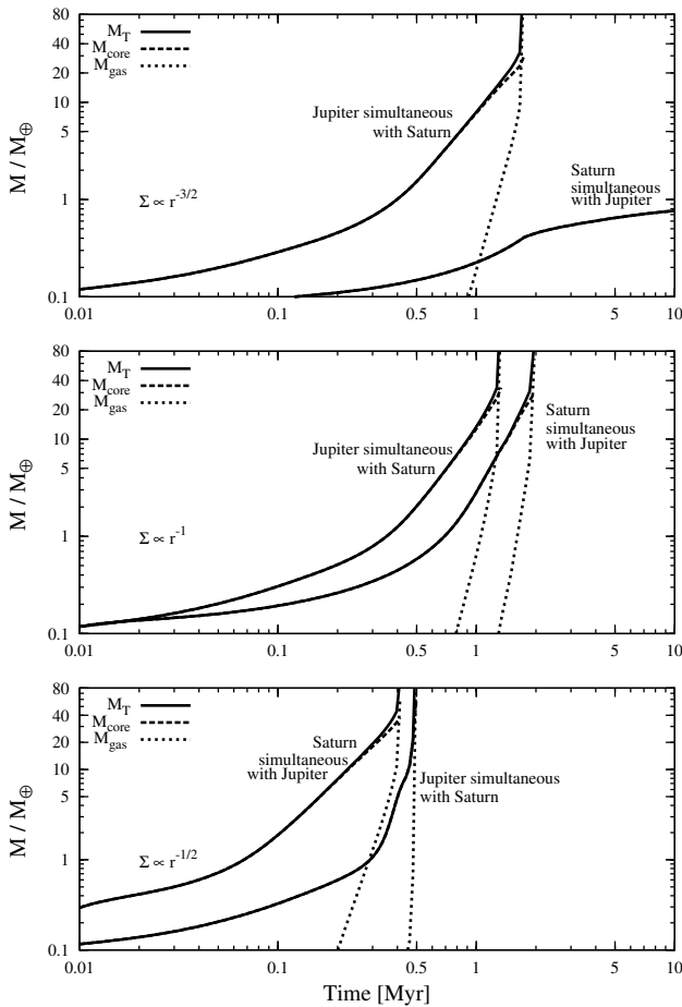
Fig. 16. Comparison of the simultaneous formation of Jupiter and Saturn for a 6 MMSN disk with different power indices ( p = 3/2; 1; 1/2 ). We see that simultaneous formation of Jupiter and Saturn changes as the power index decreases.
