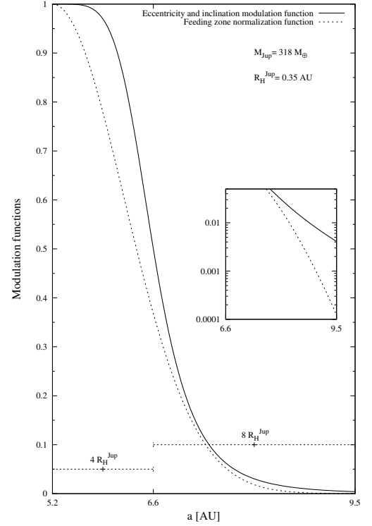
Fig. 7. Planetesimals’s eccentricity and inclination modulation function due to Jupiter gravitational stirring (Eq. 31). When Jupiter achieves its final mass, the planetesimals’s eccentricity and inclination excitation caused by Jupiter at Saturn’s location, is less than 1 % of its value at Jupiter’s orbit.
