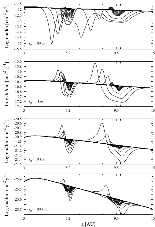
Fig. 12. Time evolution of the planetesimal density profiles for a 6 MMSN disk with power index p = 1/2 for the simultaneous formation of Jupiter and Saturn. The density wave of solids, produced by the rapid formation of Saturn is a very dispersive phenomena and strongly depends on planetesimal size. As time advances, density profiles decrease at the planets' location. Curves correspond to 0, 1 \times 10^{-7} , 1 \times 10^{-6} , 1 \times 10^{-5} , 1 \times 10^{-4} , 1 \times 10^{-3} , 0.01, 0.05, 0.1, 0.2, 0.3, 0.4, and 0.5 Myr.
