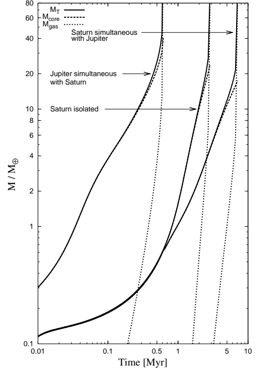
Fig. 2. Same as Fig. 1 but for a 8 MMSN. In this case, Jupiter does not inhibit Saturn formation but largely delays it.
