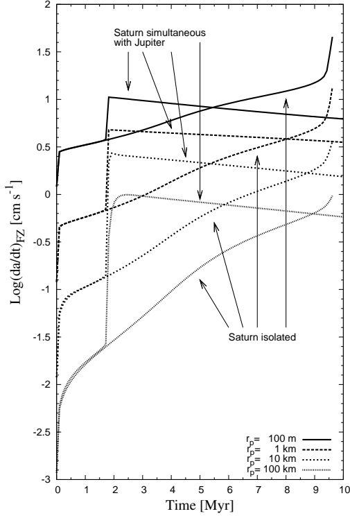
Fig. 3. The evolution of planetesimal migration mean velocities at Saturn's feeding zone for a 6 MMSN disk with power index p = 3/2 . The increase in the migration mean velocities, for the case of Saturn's simultaneous formation, is due to Jupiter's rapid formation as it reaches gaseous runaway.
