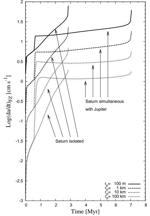
Fig. 4. Same as Fig. 3 but for the case of a 8 MMSN nebula.
