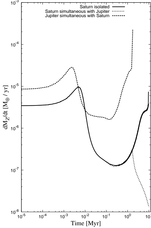
Fig. 5. A comparison of the evolution of the solid accretion rate for the simultaneous formation of Jupiter and Saturn and isolated formation of Saturn for a 6 MMSN disk with power index p = 3/2 . We see that Jupiter’s formation cuts off the solid accretion rate in the case of simultaneous formation with Saturn.
