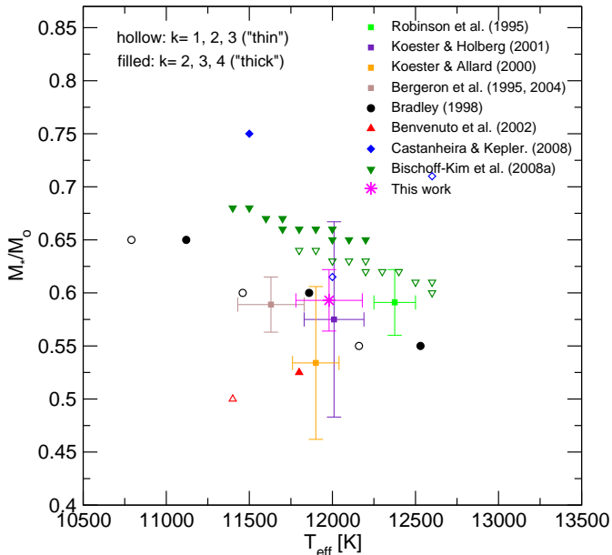
Figure 7. The location of the asteroseismological models for G117–B15A in the plane T_{\text{eff}} - M_* according to the studies carried out up to date and according to this work, as indicated with different symbols. Empty symbols correspond to solutions for which the radial order identification of the observed periods is k = 1, 2, 3 (thin H envelopes), and filled symbols are associated to solutions for which the observed periods have k = 2, 3, 4 (thick H envelopes). Also included is the location of G117–B15A according to several spectroscopic studies (filled squares). Note that Robinson et al. (1995) use \text{MLT}/\alpha = 1 model atmospheres, while the other use \text{MLT}/\alpha = 0.6 , hence they obtain lower T_{\text{eff}} values.
