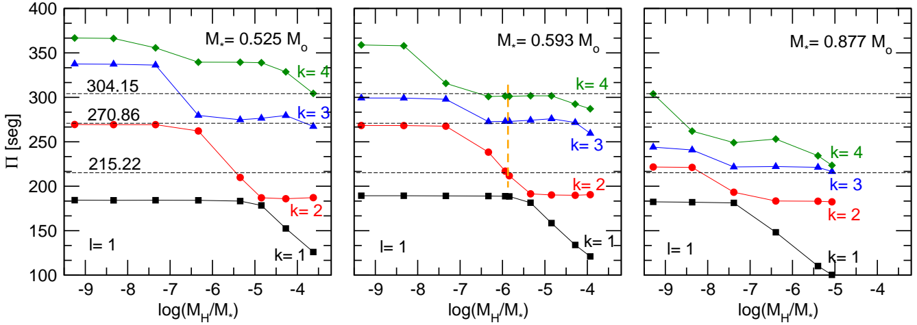
Figure 6. The periods of the modes with \ell = 1 and k = 1, 2, 3 and 4 in terms of the thickness of the H envelope corresponding to M_* = 0.525M_\odot (left panel), M_* = 0.593M_\odot (middle panel), and M_* = 0.877M_\odot (right panel). The observed periods of G117–B15A are shown with thin horizontal dashed lines. The dashed (orange) line in the middle panel indicates the match between the theoretical periods of the asteroseismological model and the periods observed in G117–B15A.
