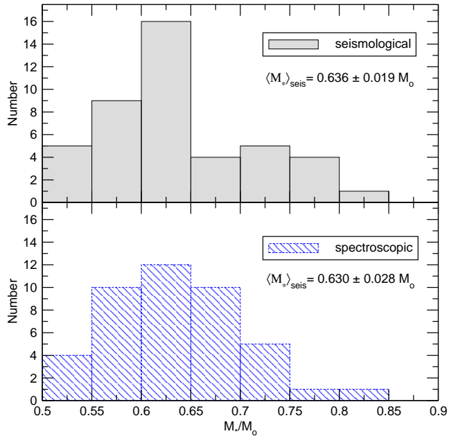
Figure 10. Histograms showing the mass distribution for the sample of 44 ZZ Ceti stars considered in this work, according to our spectroscopic inferences (lower panel) and our seismological analysis (upper panel).
