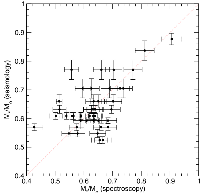
Figure 9. Comparison between the value of the stellar mass of the 44 DAVs stars analyzed in this work, according to our spectroscopic inference (x-axis) and from our asteroseismological analysis (y-axis). The red dashed line represents a perfect match between both mass estimates.
