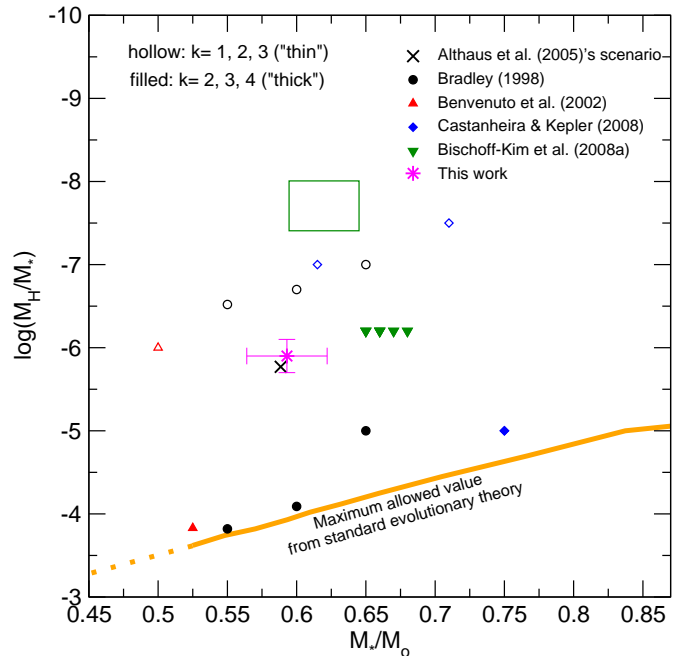
Figure 8. Similar to Fig. 7, but in the plane M_* - \log(M_{\text{H}}/M_*) . The hollow green rectangle corresponds to the thin solutions of Bischoff-Kim et al. (2008a) corresponding to an identification k = 1, 2, 3 . In the interests of comparison, the location of the post-Late Thermal Pulse remnant with a thin H envelope of the scenario of Althaus et al. (2005b) is also shown.
