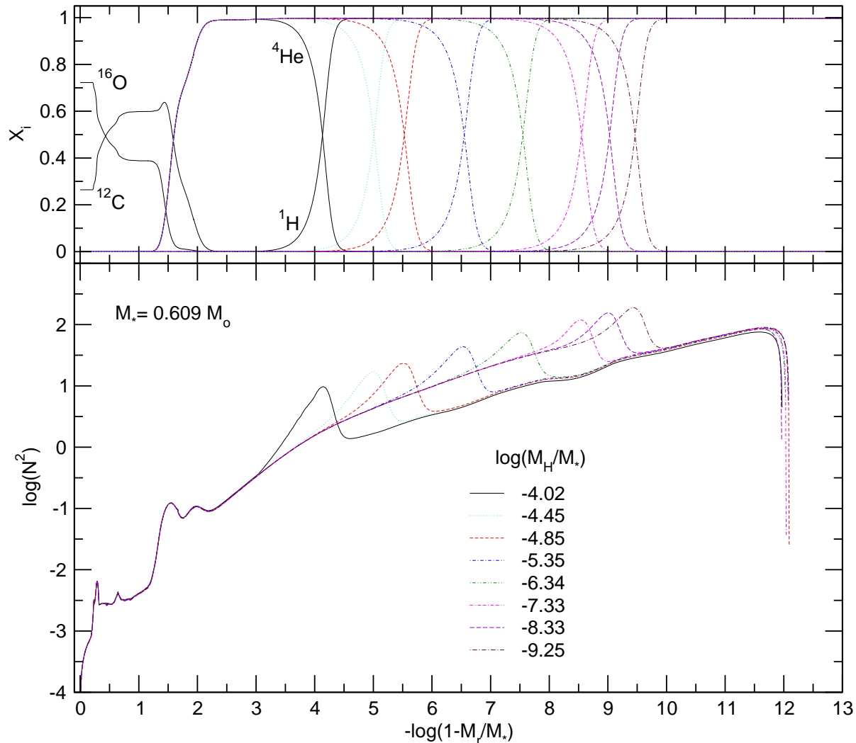
Figure 3. Upper panel: the internal chemical profiles of DA white dwarf models with M_* = 0.609M_\odot , T_{\text{eff}} \sim 12000 K, and different thicknesses of the H envelope. Only the main nuclear species are depicted. Lower panel: the run of the logarithm of the squared Brunt-Väisälä frequency for each model. Note the correspondence between the chemical transition regions (upper panel) and the resulting features in the shape of the Brunt-Väisälä frequency. For details, see the text.
