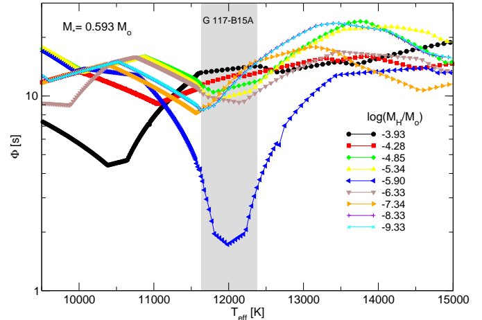
Figure 5. The quality function \Phi(M_*, M_H, T_{\text{eff}}) in terms of T_{\text{eff}} for the different values of the hydrogen thickness (shown with different colors and symbols) and a stellar mass of M_* = 0.593 M_\odot . The gray strip correspond to the effective temperature of G117–B15A according to spectroscopic analysis. Note in particular the location of the best-fit solution (the minimum of \Phi at T_{\text{eff}} \sim 12\,000 K), corresponding to the model 1 ( \ell = 1, k = 2, 3, 4 ) in Table 3.
