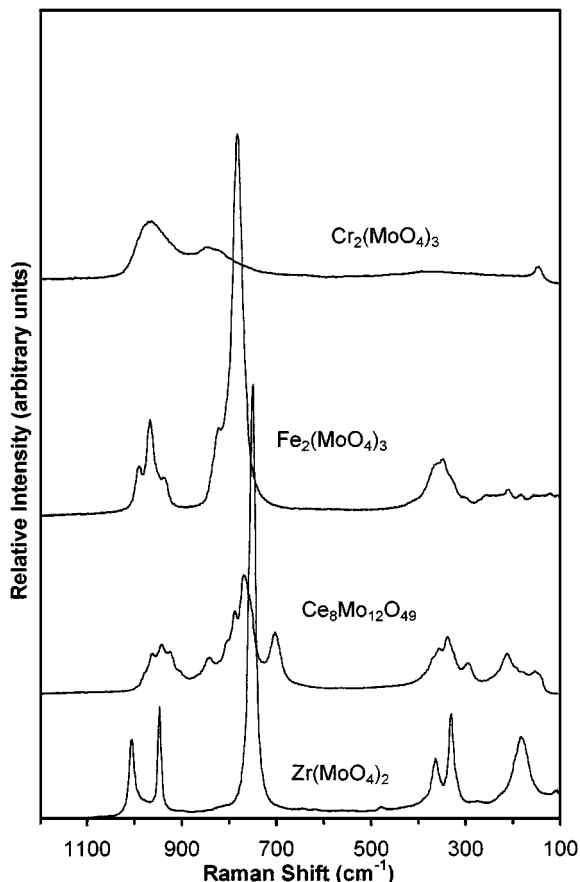
FIG. 1. Raman spectra of bulk metal molybdates.
