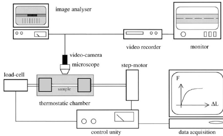
Fig. 2. Single fiber fragmentation test set up.
