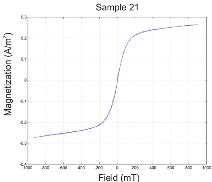
Fig. 9. Examples of most frequent shape in PCC2 hysteresis loops.
