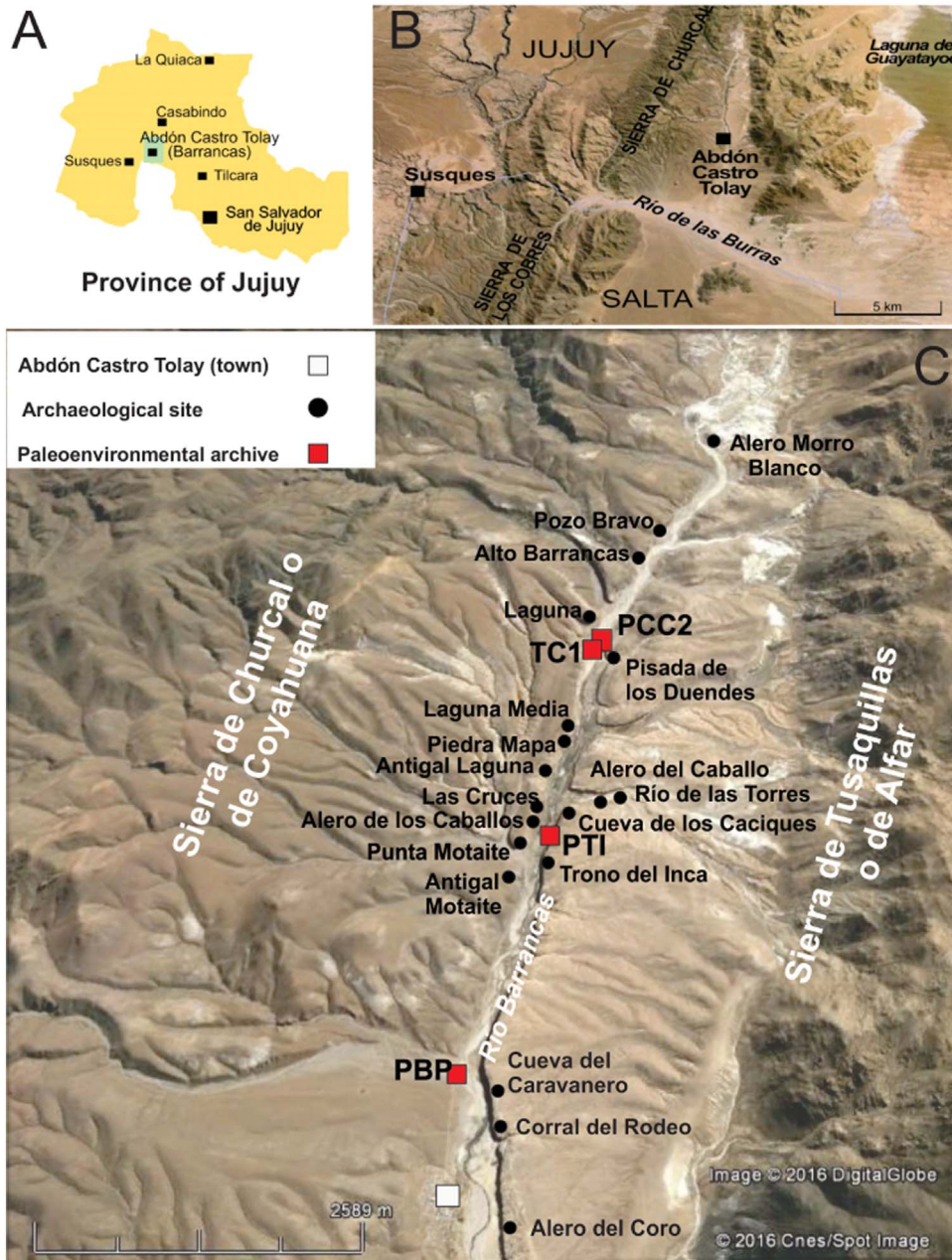
Fig. 1. A) Location of the study area within the province of Jujuy, Argentina. B) Location of the Barrancas river basin and Barrancas-Abdon Castro Tolay. C) Map of archaeological sites and paleoenvironmental archives in the Barrancas river basin. TC1: Testigo Cruces 1. PCC2: Cruces 2 profile. PTI: Trono del Inca profile. PBP: Barrancas Pueblo profile. Image source: Google Earth. 23°18'42.09"S; 66°03'24.81"W. October 16, 2014 (accessed April 11, 2017).
