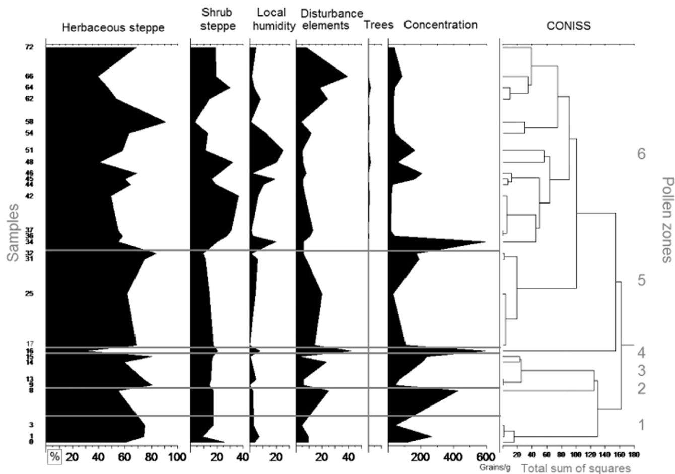
Fig. 14. Pollen ecological spectra, zonation (CONISS) and pollen concentration.
