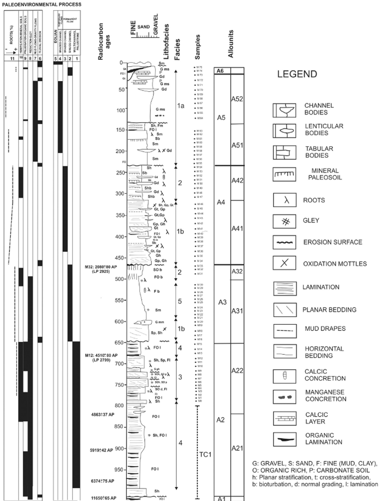
Fig. 5. PCC2 lithofacies and overall stratigraphy. Allunits A1 and A1.2. correspond to the Cruces 1 core (TC1, Morales et al., this volume).
