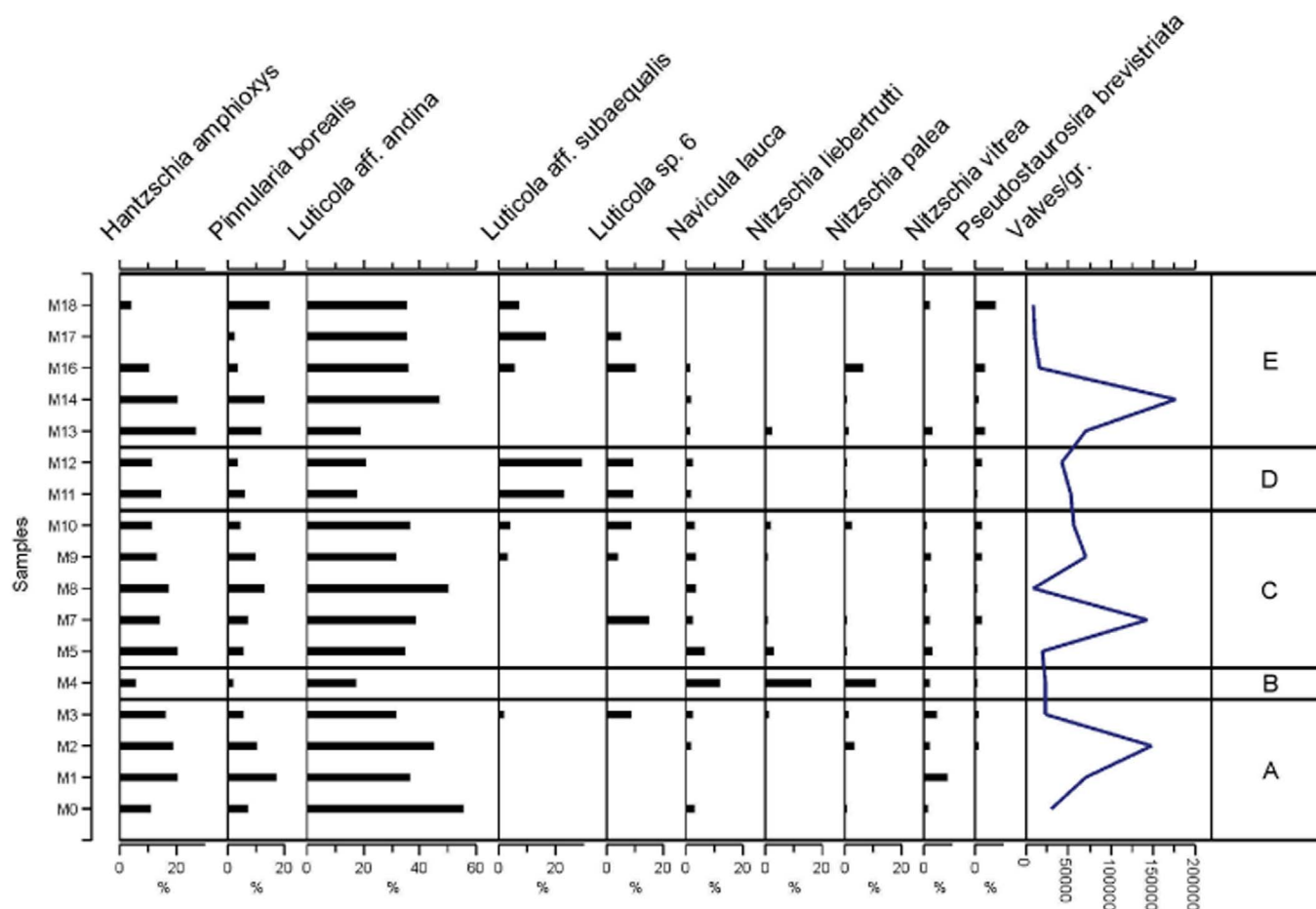
Fig. 11. Most frequent (> 5%) diatoms taxa, diatoms concentrations and floristic zonation.
