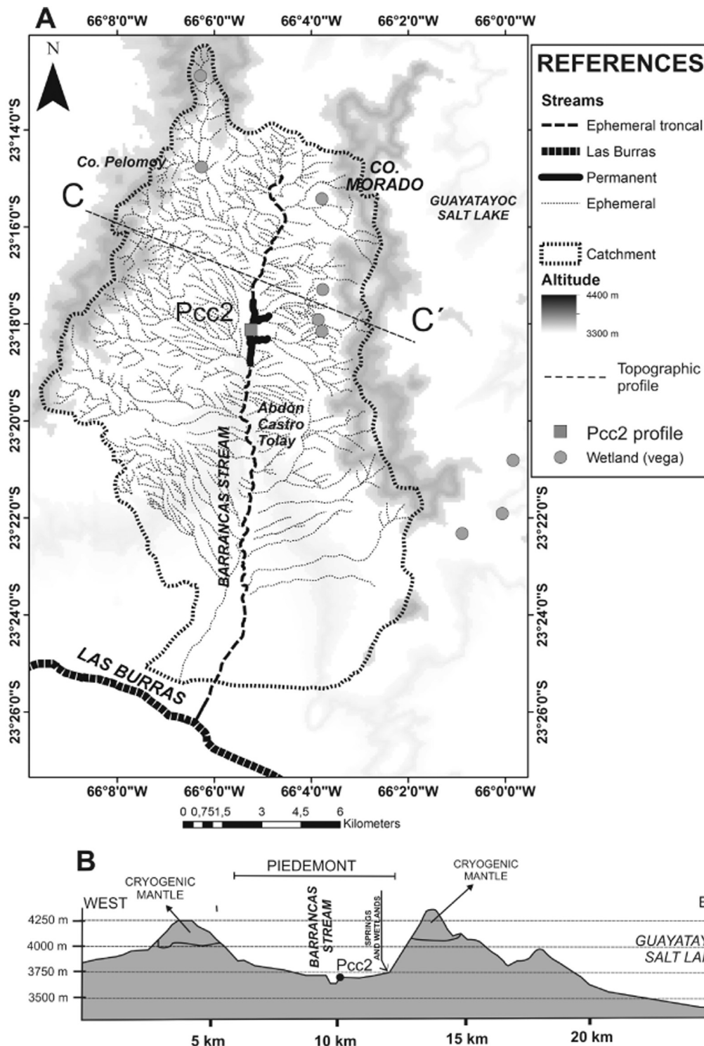
Fig. 2. A. The Barrancas river basin. B. West to east profile (C – C' in panel A) of the Barrancas area.
