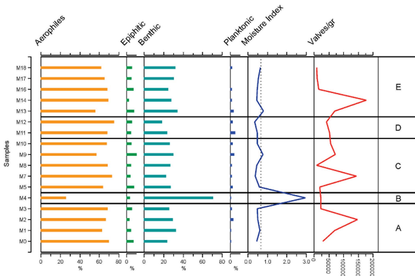
Fig. 12. Diatom life-form affinity spectra, moisture index and diatoms concentrations.
