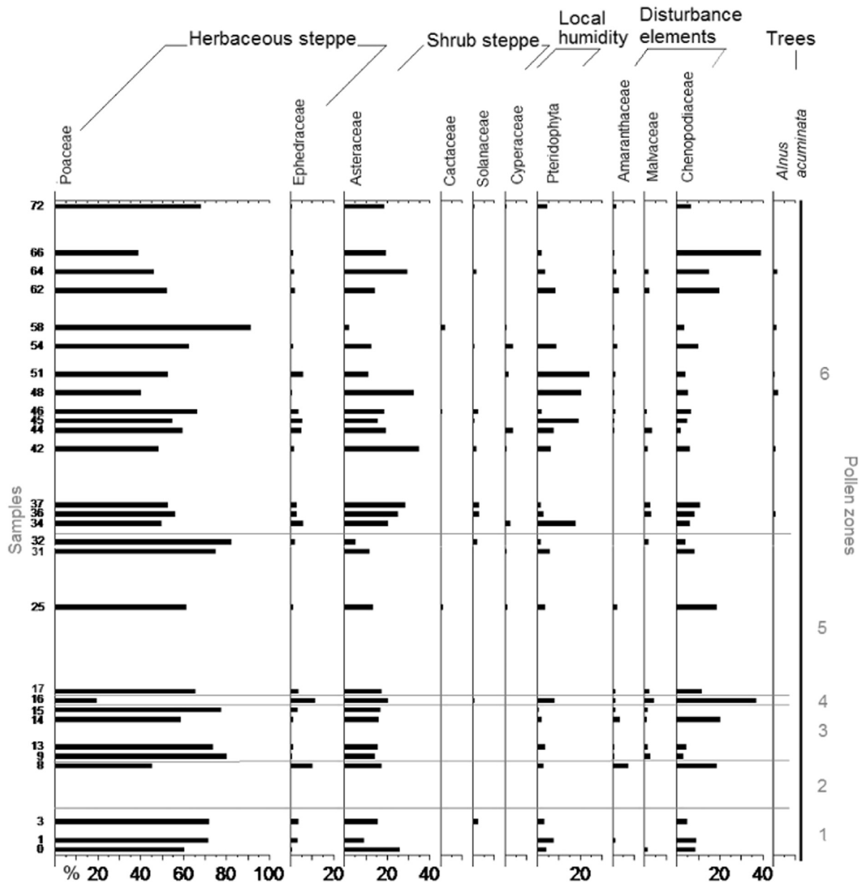
Fig. 13. Most frequent pollen taxa in the PCC2 sequence.
