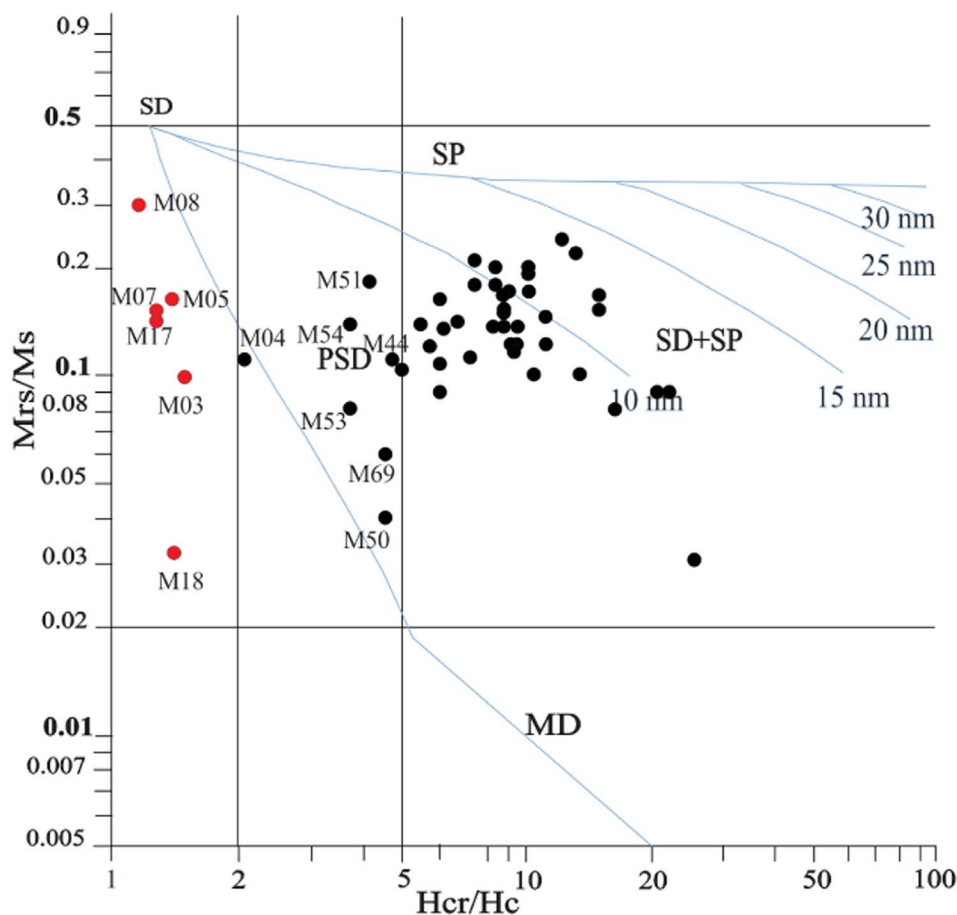
Fig. 10. Day Plot (Mrs/Ms vs Hcr/Hc) of PCC2 samples. Red dots represent mixed particle size assemblies (SD + MD). (For interpretation of the references to color in this figure legend, the reader is referred to the web version of this article.)
