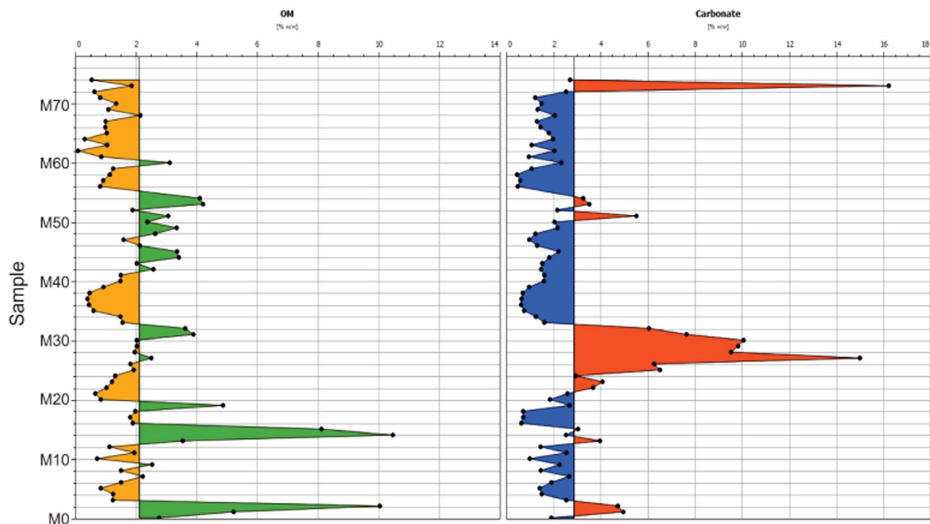
Fig. 7. OM and carbonate content (% dry w/w) obtained by LOI. Values above the mean of the series is represented in green or red; values below the mean is represented in yellow or blue. (For interpretation of the references to color in this figure legend, the reader is referred to the web version of this article.)
