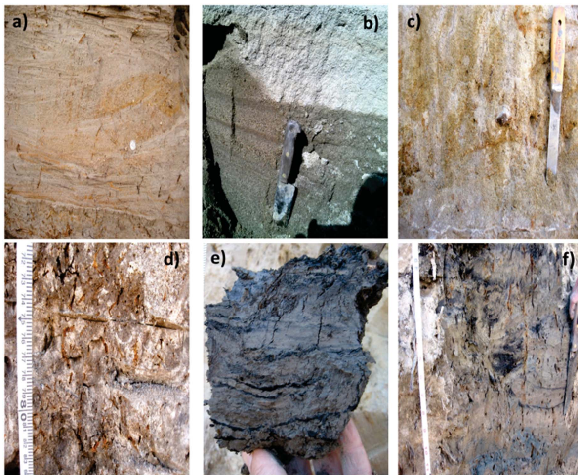
Fig. 6. Examples of lithofacies described in Table 1. a) Lithofacies Gh and GP. 3.5 m deep; b) very coarse, upward-fining, laminated sands (lithofacies Sd, Sh with Fl). Light colors, no bioturbation; c) massive sands with disperse gravel (lithofacies Gmc), 5 m deep; d) massive, bioturbated clays, with root traces and gleyzation (lithofacies Fb), 4.5 m deep; e) lithofacies FOI, greenish to grayish clays laminated with OM, 6.8 m deep; f) Brown and greenish clays with lenticular OM laminae and vegetal macroremains (lithofacies FOIb) at 5.6 m deep. (For interpretation of the references to color in this figure legend, the reader is referred to the web version of this article.)
