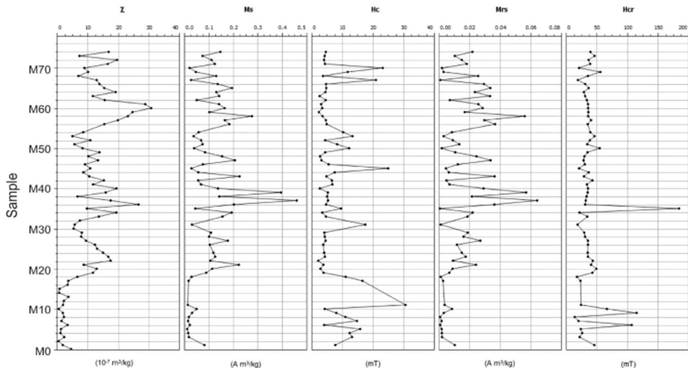
Fig. 8. Magnetic properties of PCC2 sediments.
