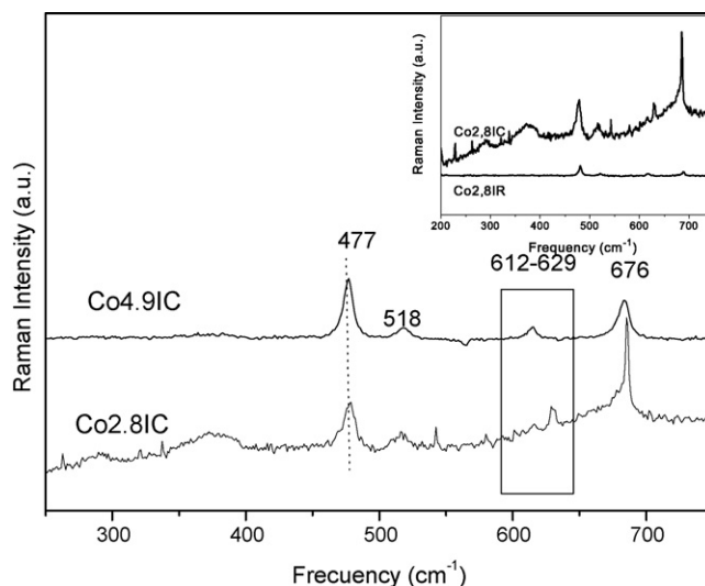
Fig. 7. Laser Raman spectra of calcined Co2.8IC and Co4.9IC. Inset: Co2.8IC and Co2.8IR Laser Raman spectra.
