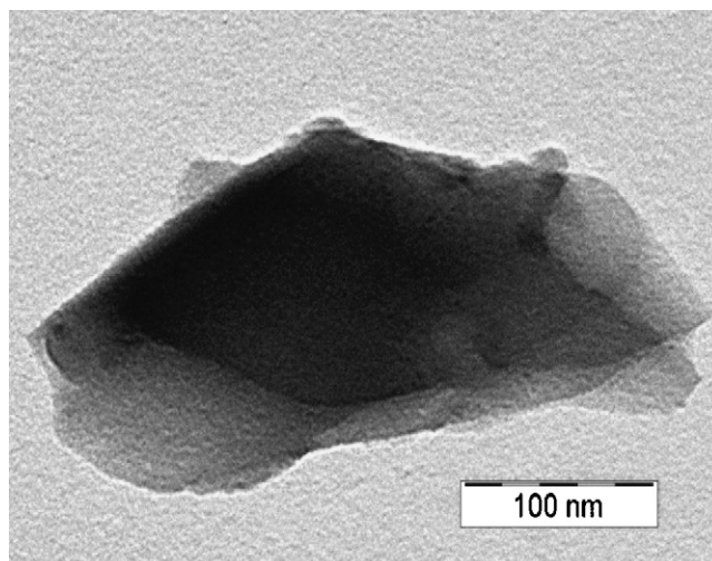
Fig. 5. Transmission electron micrography of sample Co4.9IC.
