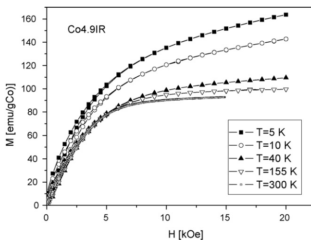
Fig. 9. M vs. H curves for sample Co4.9IR at different temperatures.
