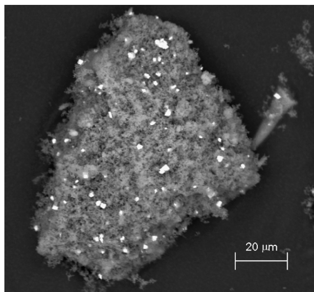
Fig. 4. Micrography of Co 4.9 IC taken at 1500 \times . The bright spots are Co oxide particles.
