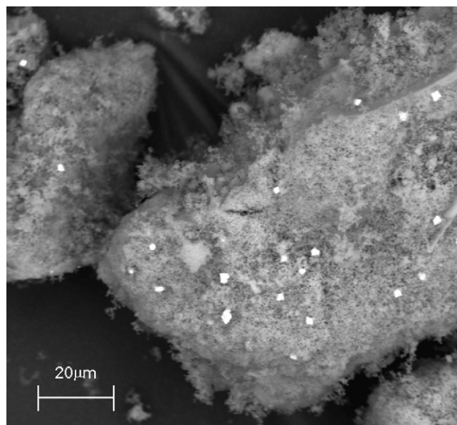
Fig. 3. Micrography of Co 2.8 IC taken at 1500 \times . The bright spots are Co oxide particles.
