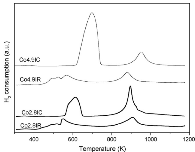
Fig. 6. TPR profiles of Co2.8IC, Co2.8IR, Co4.9IC and Co4.9IR.
