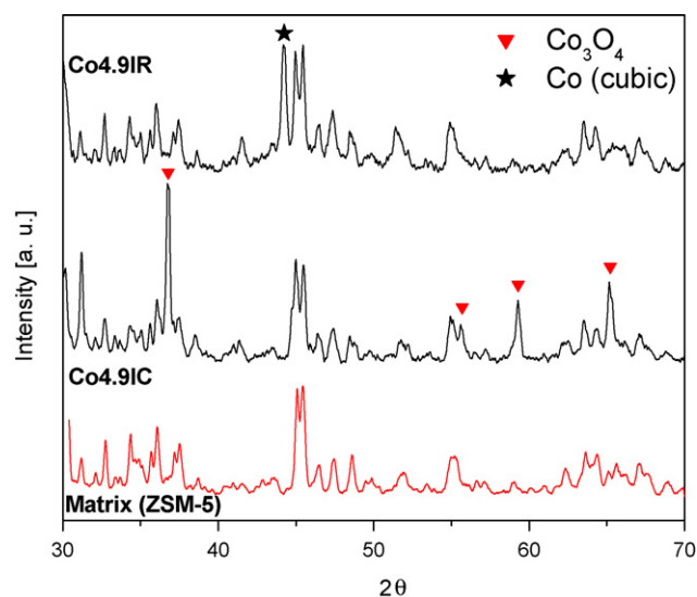
Fig. 2. Diffraction patterns of samples Co4.9IC and Co4.9IR. The bottom pattern corresponds to the matrix ZSM-5.
