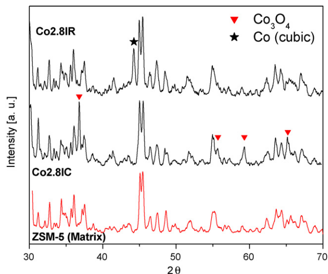
Fig. 1. Diffraction patterns of samples Co2.8IC and Co2.8IR. The bottom pattern corresponds to the matrix ZSM-5.
