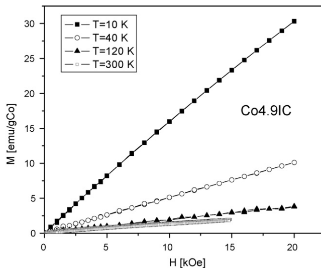
Fig. 8. M vs. H curves for sample Co4.9IC at different temperatures.
