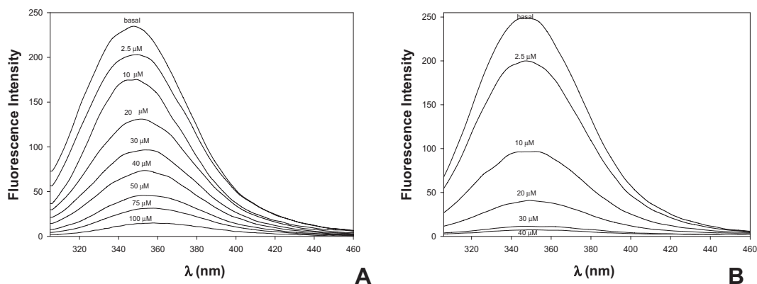
Fig. 11. The fluorescence spectra of BSA at various concentrations of baicalin (A) and VIVO(baic) (B). \lambda_{\text{ex}} = 280 \text{ nm} , [\text{BSA}] = 6 \mu\text{M} , T = 310 \text{ K} .
