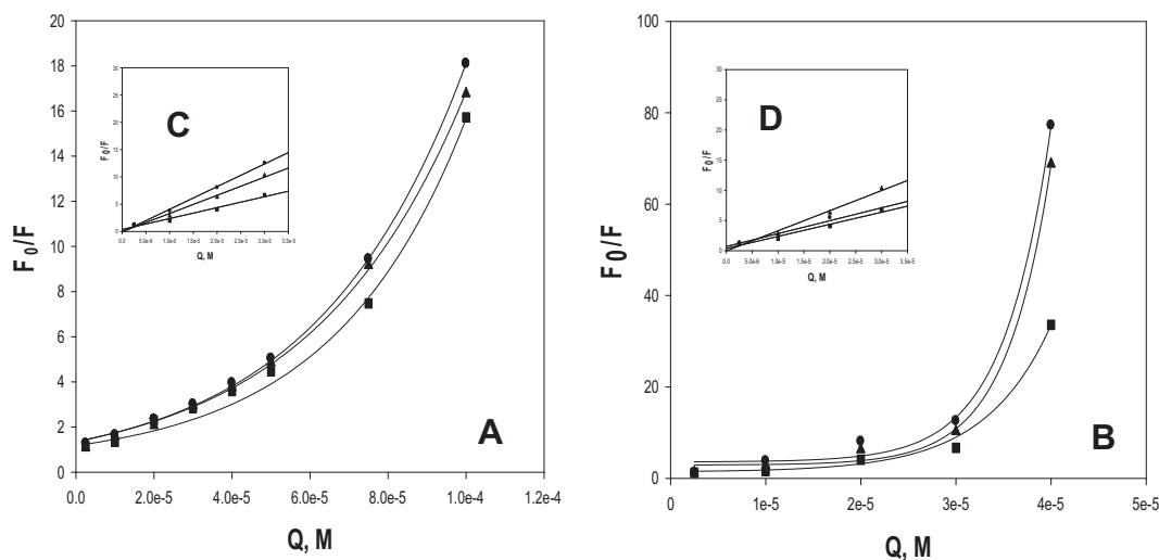
Fig. 12. Plots of F_0/F vs [Q] for BSA with baicalin (A) and VIVO(baic) (B) at different temperatures ((●), 298 K; (▲), 303 K; (■), 310 K), \lambda_{\text{ex}} = 280 \text{ nm} . Inset: F_0/F vs [Q] of baicalin (C) and VIVO(baic) (D).
