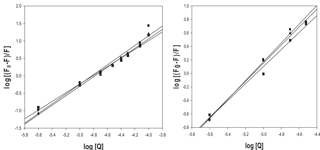
Fig. 13. Plots of \log [(F_0 - F)/F] vs. \log [Q] for the baicalin-BSA system (A) and V^{IV}O(baic) -BSA system (B): (●), 298 K; (▲), 303 K; (■), 310 K, [BSA] = 6 \mu M , \lambda_{ex} = 280 .
