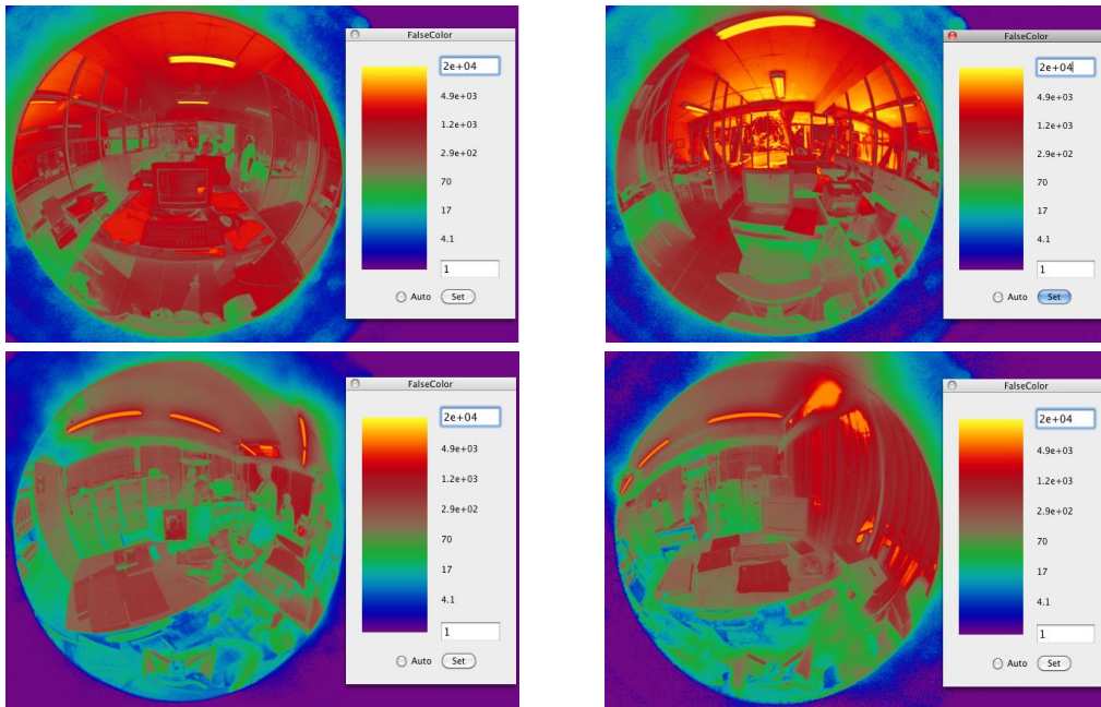
Figure 2 - Luminance mappings of workstations where discomfort glare was predicted. a. Case 9. b. Case 10. c. Case 11. d. Case 12.
