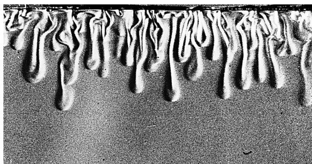
Fig. 9. Schlieren view of the CO 2 convective dynamics at t = 10 min in a solution of NaOH 2.000 \times 10^{-2} mol/L. The field of view is 11.7 cm wide.
