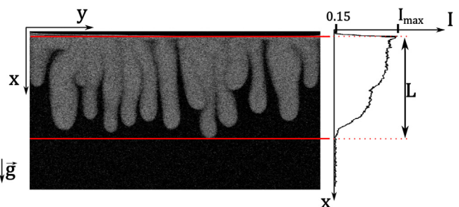
Fig. 4. Processed image of \text{CO}_2 fingers in BP solution at t = 30 min and corresponding TAP along the x axis. The finger length L is computed as the length of the region where TAP decreases from its maximum value I_{max} (the interface) to 0.15.
