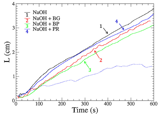
Fig. 11. Full curves: temporal evolution of finger length L , computed from the Schlieren view of \text{CO}_2 convective dynamics in NaOH solutions containing a color indicator or not. Dashed curve: fingers growth visualized directly by color changes of PR. The concentration of NaOH and color indicators are 2.000 \times 10^{-2} mol/L and 2.50 \times 10^{-3} mol/L, respectively. Each curve represents the average of 5 experiments. (For interpretation of the references to color in the text, the reader is referred to the web version of this article.)
