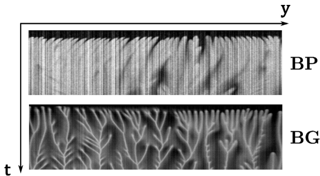
Fig. 3. Space–time maps of the location of fingers at a fixed depth (2 mm below the interface) as a function of time in BP (up) and BG (down) solutions. The concentration of color indicator is 1.00 \times 10^{-4} mol/L in both cases. The field of view is 13.7 cm wide and time is running downwards, t_{max} = 30 min.
