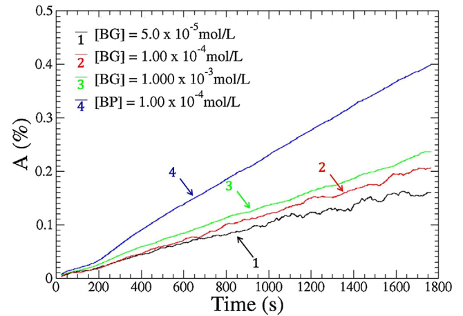
Fig. 6. Temporal evolution of relative area A of the convective pattern in BP ( 1.00 \times 10^{-4} mol/L) and BG ( 5.0 \times 10^{-5} mol/L; 1.00 \times 10^{-4} mol/L; and 1.000 \times 10^{-3} mol/L) solutions. Each curve represents the average of 5 experiments.
