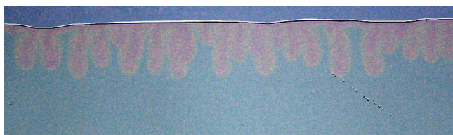
Fig. 7. Convective pattern induced by CO 2 dissolution in water containing a universal color indicator. This indicator is sensitive to pH variations in a range from 4 to 10 and is able to highlight different iso-pH zones inside the fingers. (For interpretation of the references to color in this figure legend, the reader is referred to the web version of this article.)
