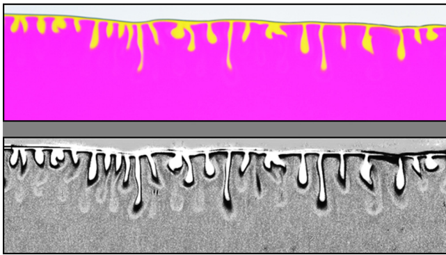
Fig. 10. Comparison of \text{CO}_2 convective dynamics at t=300 s in a solution of NaOH ( 1.000 \times 10^{-2} mol/L) containing phenol red ( 5.0 \times 10^{-4} mol/L) by direct visualization of color changes (up) and by Schlieren visualization (down). (For interpretation of the references to color in this figure legend, the reader is referred to the web version of this article.)
