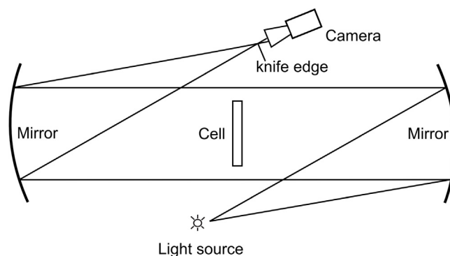
Fig. 8. Schematic of the Z-type Schlieren system used to visualize buoyancy-driven convection of CO 2 in NaOH solutions. Our set-up is composed of two 20 cm diameter mirrors with 1 m focal lengths. The Hele-Shaw cell is placed between the two mirrors and a CCD monochromatic camera records the dynamics at successive times.
