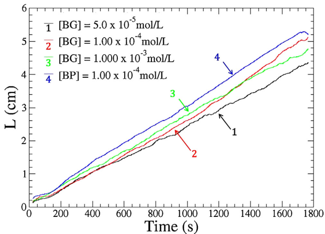
Fig. 5. Temporal evolution of finger length L of \text{CO}_2 convective dynamics in BP ( 1.00 \times 10^{-4} mol/L) and BG ( 5.0 \times 10^{-5} mol/L; 1.00 \times 10^{-4} mol/L; and 1.000 \times 10^{-3} mol/L) solutions. Each curve represents the average of 5 experiments.
