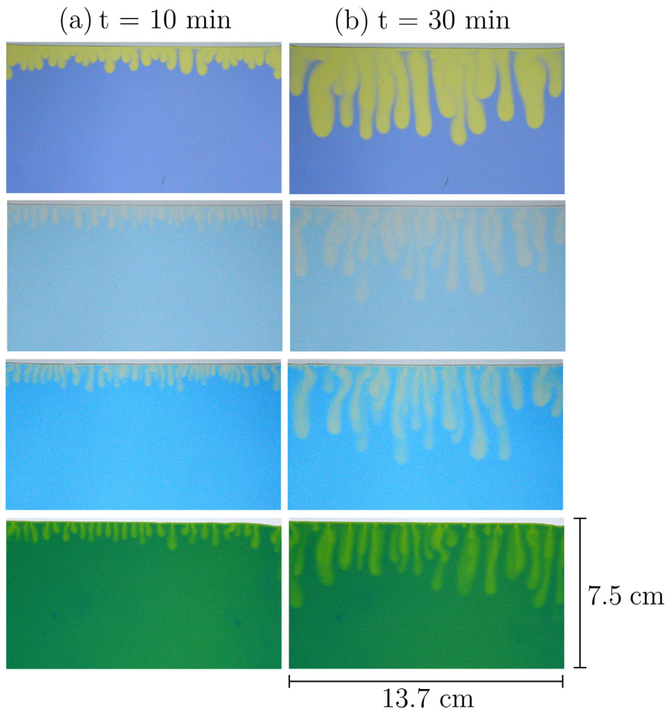
Fig. 2. Development of density driven instability at (a) t = 10 min and (b) t = 30 min, induced by the dissolution of \text{CO}_2 at atmospheric pressure in water containing from top to bottom: bromocresol purple 1.00 \times 10^{-4} mol/L, bromocresol green 5.0 \times 10^{-5} mol/L; 1.00 \times 10^{-4} mol/L; and 1.000 \times 10^{-3} mol/L. The field of view focuses on the lower aqueous phase. Experiments are carried out at room temperature. (For interpretation of the references to color in this figure legend, the reader is referred to the web version of this article.)
