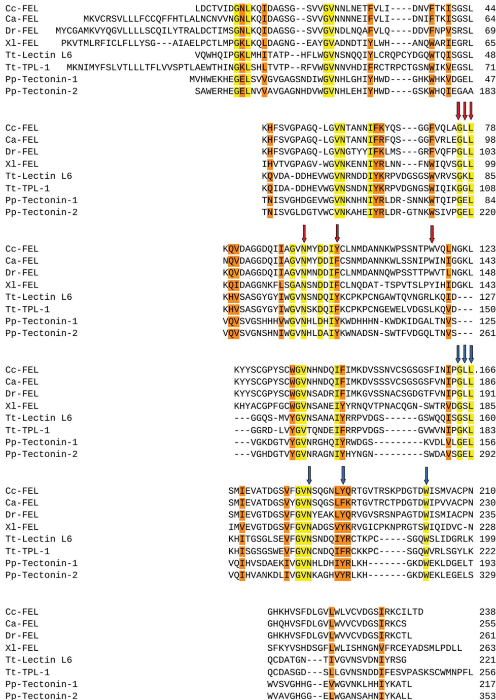
Figure 6 Amino-acid sequence homology of carp FEL: comparison with proteins encoded by homologous genes in fish and amphibians and with members of the invertebrate lectin family. The sequences were aligned using ClustalW (Thompson et al. , 1994; Larkin et al. , 2007) and correspond to the following lectins (UniProt codes are given in parentheses): Cc-FEL (P68512), carp ( Cyprinus carpio ) FEL; Ca-FEL (Q78BR1), goldfish ( Carassius auratus ) FEL; Dr-FEL (A8E5B4), zebrafish ( Danio rerio ) FEL; Xl-FEL (A8E602), African clawed frog ( Xenopus laevis ) FEL; Tt-Lectin L6 (P82151), Japanese horseshoe crab ( Tachypleus tridentatus ) lectin L6; Tt-TPL-1 (Q9NB63), galactose-binding protein from Japanese horseshoe crab ( T. tridentatus ); Pp-Tectonin-1 (O61063), tectonin-1 from the slime mould Physarum polycephalum ; Pp-Tectonin-2 (O61064), tectonin-2 from the slime mould P. polycephalum . The six blocks correspond to the six blades of carp FEL. The residues that are conserved in all of the sequences are contained in yellow boxes, while those that have strongly similar properties (scoring >0.5 in the Gonnet PAM 250 matrix; Gaston et al. , 1992) are contained in orange boxes. Red arrows identify the residues of cFEL involved in ligand binding in site \alpha and blue arrows those in site \beta .
