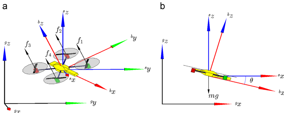
Fig. 1. Ar.Drone quadrotor: (a) 6-DOF model, with the reference system and the abstract control inputs f_i associated with it. The inertial, spatial and body frame are (g) , (s) and (b) , as indicated by the left superscript in the axes x , y and z . (b) The PVTOL model of the quadrotor.
