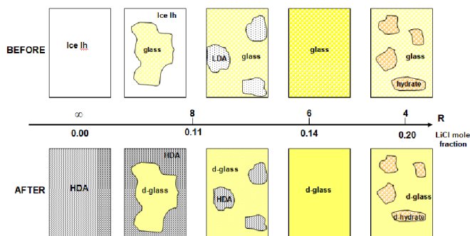
FIG. 6. Scheme of the LiCl - \text{H}_2\text{O} system before and after pressurization at 77 K at some representative salt concentrations in the water- and salt-dominated regimes.
