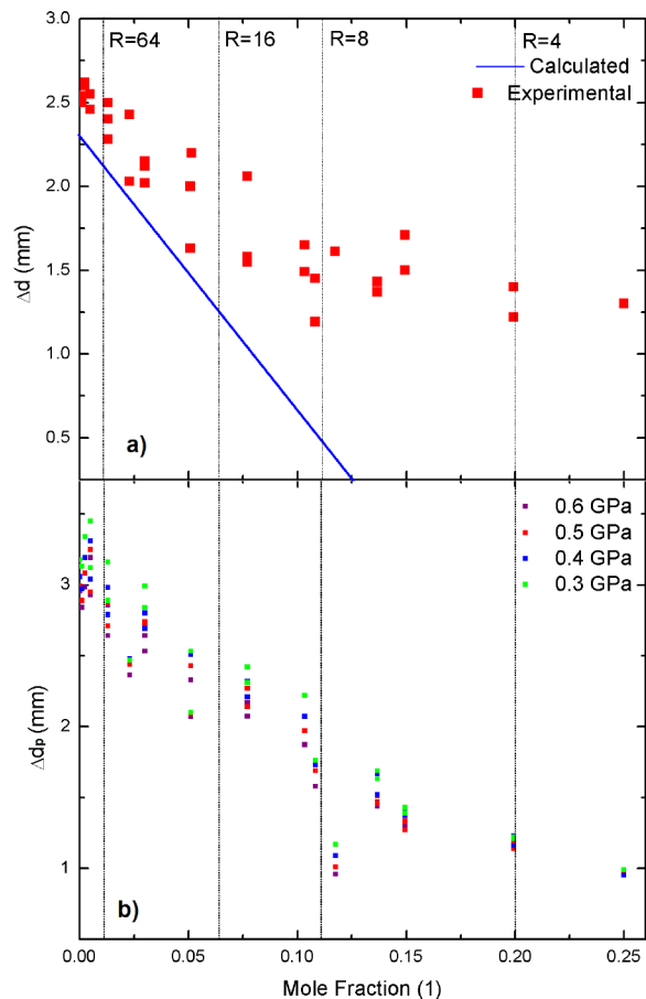
FIG. 4. (a) Piston displacement as a function of salt concentration. Blue line shows calculated values (see text). (b) Values of \Delta d_p (see figure 2) at different pressures as a function of salt concentration. Single points represent independent measurements.
