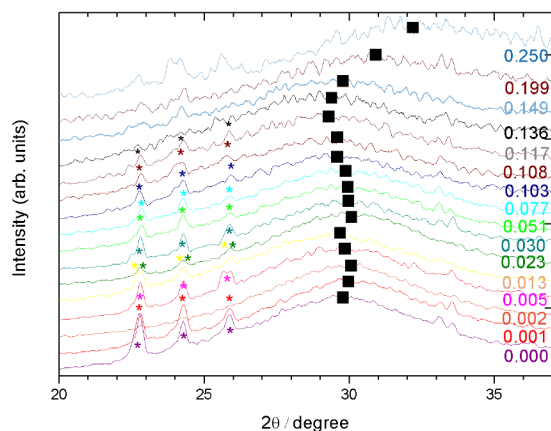
FIG. 7. XRDs indicating the shift of the corresponding halo maxima as a function of LiCl mole fraction.
