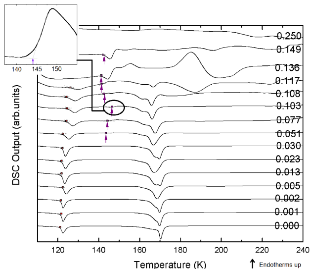
FIG. 9. DSC scans (heating rate 30 K/min) of recovered samples after pressurization to 1.6 GPa for concentrations from x = 0 to x = 0.25 . Red points indicate the onset temperature for HDA \rightarrow LDA transition and violet arrows indicate T_g onset temperature in samples of concentrations higher than x = 0.051 .
