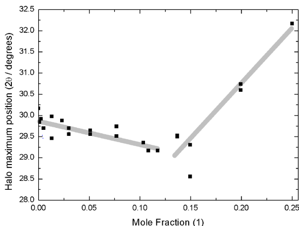
FIG. 8. Halo maximum position as a function of LiCl mole fraction. Broad lines indicate trends as guide for the eye. Single points represent individual measurements.
