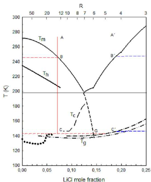
FIG. 1. Phase diagram of the LiCl-H 2 O system. T_m : melting line; T_s : solubility curves of the different hydrates (LiCl. x H 2 O); T_g : glass transition temperature (dotted line from Ref. [15]; dash-dot line from Ref. [7]; dash-dot-dot line from [16]). T_c , ice crystallization line from ref. [16]; T_h , homogeneous nucleation line from ref. [9] (data for NaCl can also be used for LiCl since the T_h was shown to be a colligative property [9]). E indicates the eutectic point of the mixture, the dashed line is an assumed extrapolation of the ice melting curve in the supercooled region, and G represent the maximally freeze-concentrated phase, located close to R=6 [16].
