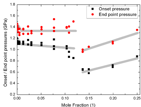
FIG. 3. Onset and end point pressures for transformations of LiCl - H 2 O samples upon pressurization at 77 K. Values are extracted from the intersections of the tangents in Fig.2. The broad lines are guides to the eye. Single points represent independent measurements.
