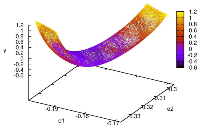
Figure 3. A cut with the plane x = 0 ( u > 0 ) of a partially chaotic orbit from the chain shown in Fig. 2. It is shown in the 3D space ( e_1 , e_2 , y ) with the fourth dimension z given by the colour scale in the electronic version. (A colour version of this figure is available in the online version.)
