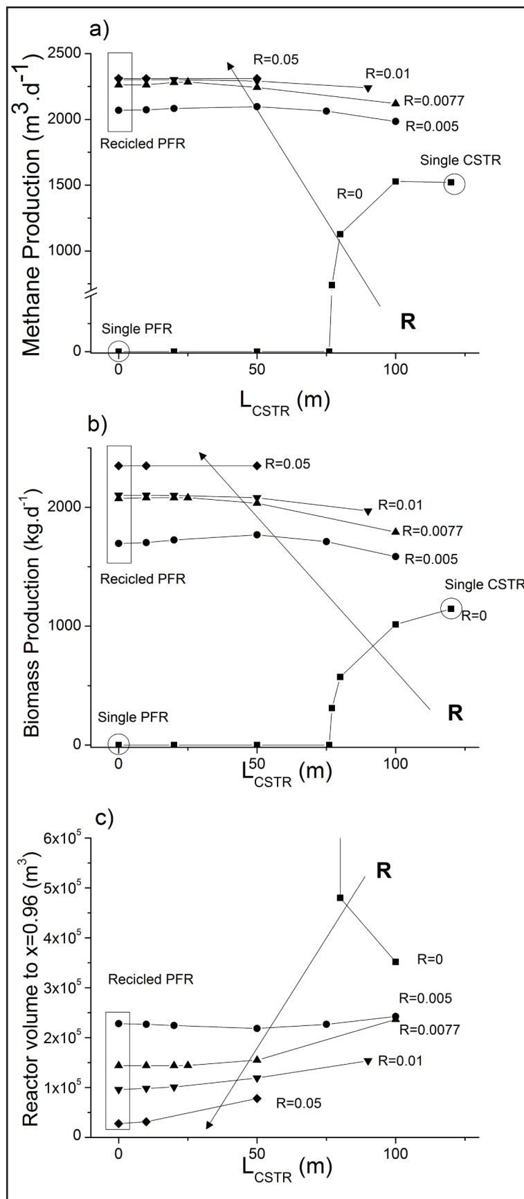
Figure 5. a) methane, b) biomass production, and c) the Reactor volume necessary to attain x=0.96 vs. L_{CSTR} using R as parameter.
