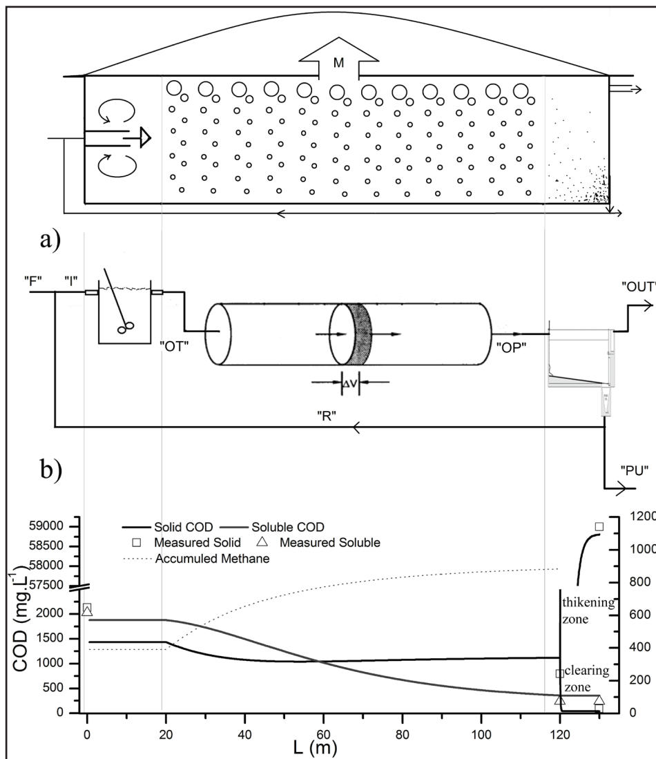
Figure 2. Solid and soluble biodegradable organic fractions and methane measured during laboratory assay. The kinetic fitting also is shown as solid lines.
