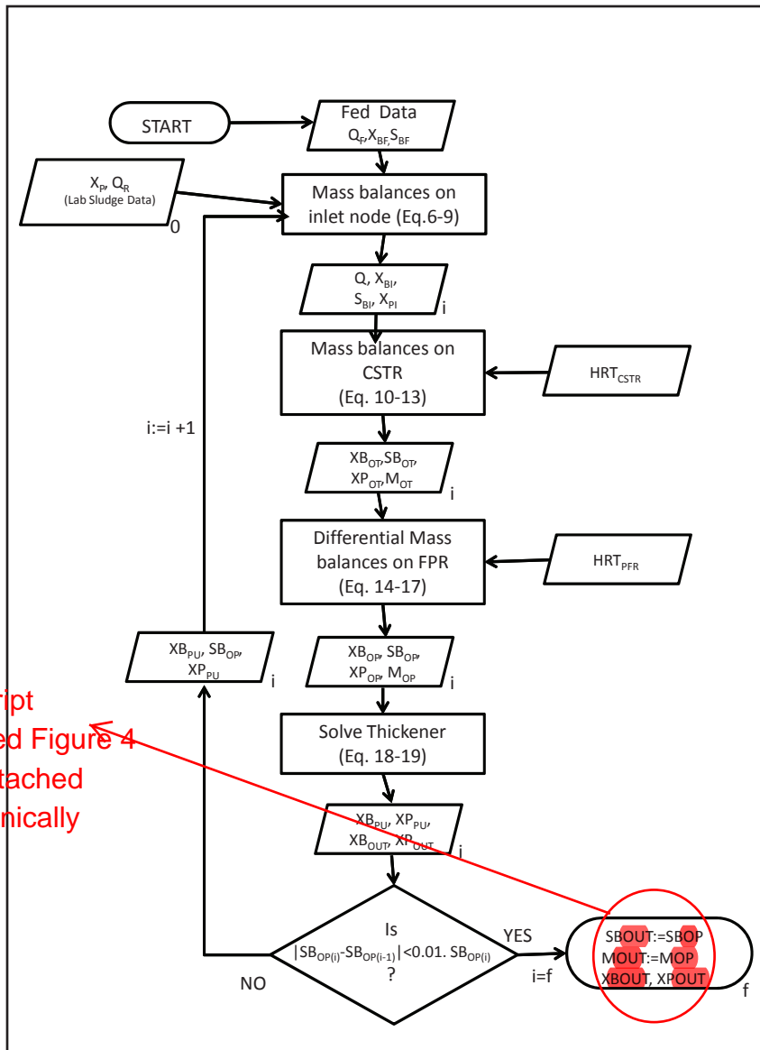
Figure 4. Algorithm structure.
