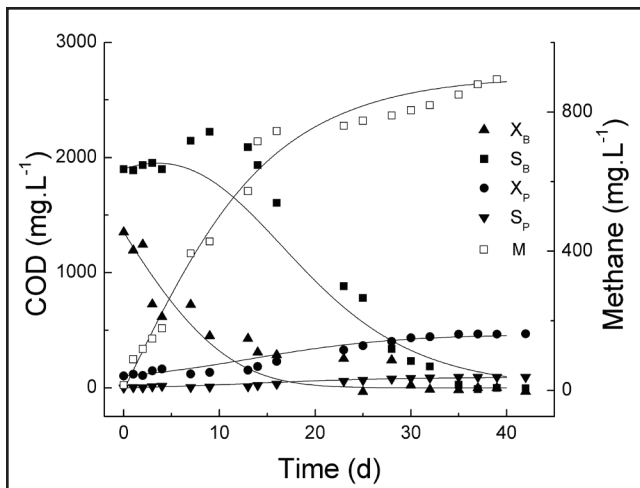
Figure 2. Solid and soluble biodegradable organic fractions and methane measured during laboratory assay. The kinetic fitting also is shown as solid lines.
