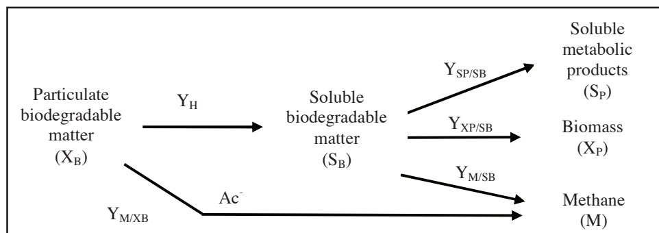
Figure 1. Proposed kinetic reaction scheme.
