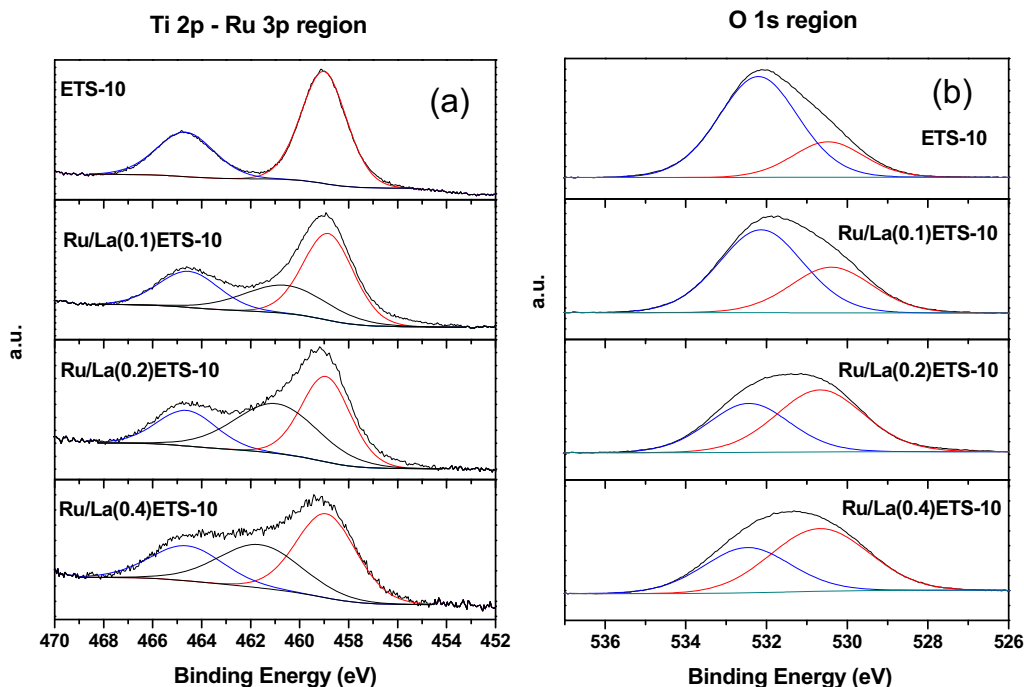
Fig. 8. XPS spectra of Ti 2p–Ru 3p (a) and O 1s (b) regions for Ru/catalysts compared with ETS-10.
