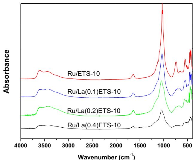
Fig. 6. FTIR spectra of Ru/La(X)ETS-10 and Ru/ETS-10 catalysts.
