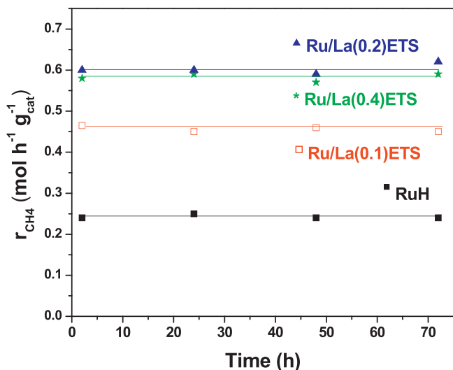
Fig. 2. Stability test of the catalysts after reduction at 550 °C in the fixed-bed reactor (reaction temperature = 550 °C, P = 100 kPa, W/F = 4.3 \times 10^{-6} g h cm –3 (feed composition: P_{CH_4} : P_{CO_2} : P_{Ar} = 1 : 1 : 1 )).
