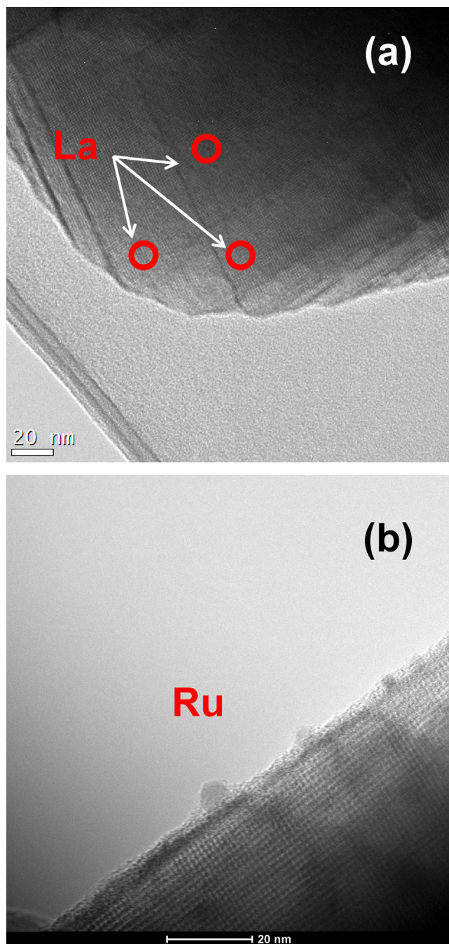
Fig. 7. TEM images of La(0.4)ETS-10 support (a) and reduced Ru/La(0.4)ETS-10 catalyst (b).
