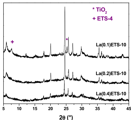
Fig. 3. XRD patterns of La(X)ETS-10 supports with different lanthanum contents.
