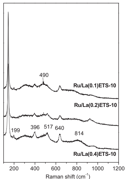
Fig. 5. Laser Raman spectra of Ru/La(X)ETS-10 fresh catalysts.
