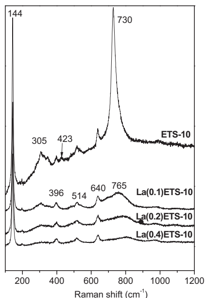
Fig. 4. Laser Raman spectra of La(X)ETS-10 supports compared with ETS-10.
