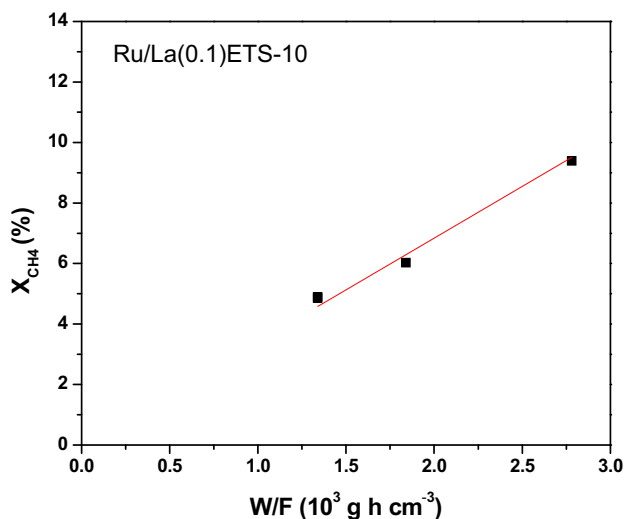
Fig. 1. CH 4 conversion as a function of residence time ( W/F ) for Ru/La(0.1)ETS-10 varying total flux between 90 and 187 cm 3 min -1 (reaction temperature = 550 °C, P = 100 kPa, feed composition: P_{\text{CH}_4} : P_{\text{CO}_2} : P_{\text{Ar}} = 1 : 1 : 1.1 ).
