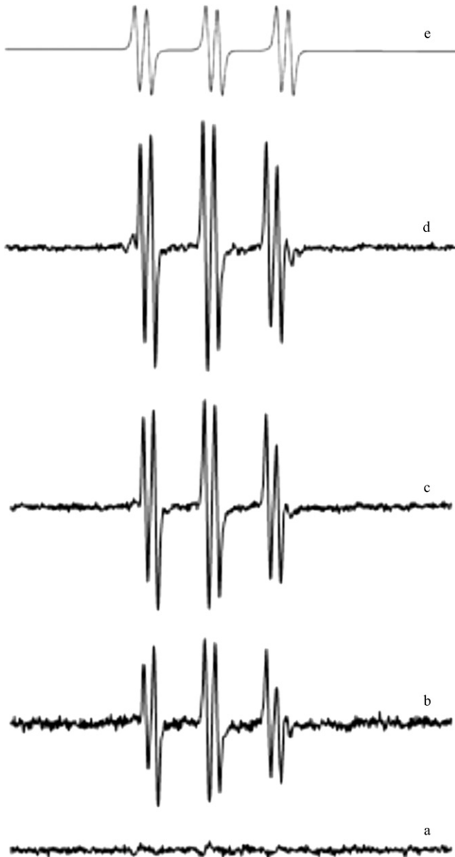
Fig. 6. Lipid radical detection by EPR in digestive gland of A. atra atra from Nuevo Gulf in winter of 2011: (a) EPR spectra of dimethylsulfoxide, (b) typical EPR spectra of digestive gland from Storni Dock, (c) typical EPR spectra of digestive gland from Folias Wreck, (d) typical EPR spectra of digestive gland from Punta Cuevas and (e) computer-simulated spectrum employing the following spectral parameters g=2.005 and a_H=1.8 G, are shown.
