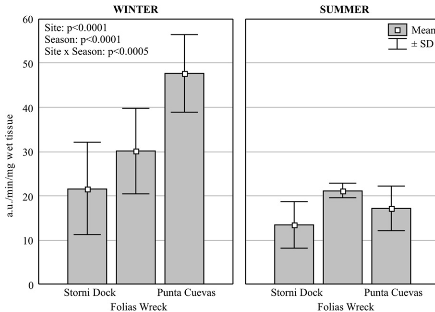
Fig. 5. ROS production in digestive gland of A. atra atra from Nuevo Gulf ( n=6 ). The statistical significance was analyzed by two-way ANOVA test with site and season as factors.
