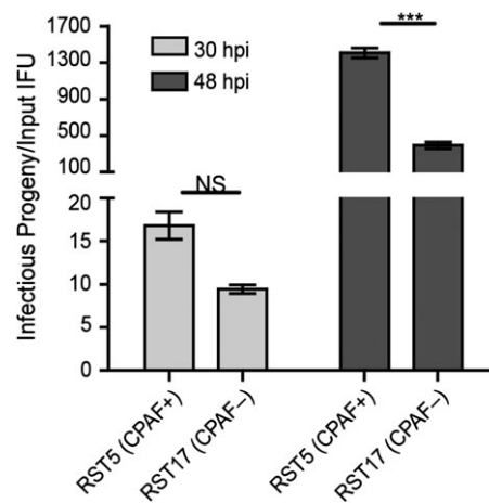
Fig. 2 Chlamydia trachomatis mutants deficient in CPAF expression are impaired for the generation of infectious progeny. Vero cells were infected with the indicated strains at an MOI = 0.3, and infectious progeny released per input IFU was calculated at 30 hpi and 48 hpi. RST17 (CPAF − ) mutants produce a threefold lower yield of infectious units compared with RST5 (CPAF + ) bacteria at 48 hpi. Three independent experiments, SEM, two-way ANOVA with Bonferroni post hoc , *** P < 0.001.
