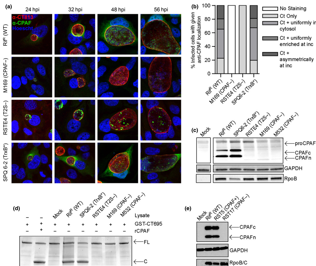
Fig. 1 Identification of Chlamydia trachomatis strains deficient in CPAF secretion or expression. (a–b). CPAF fails to accumulate in the cytoplasm of cells infected with a T2S-deficient mutant and is not detectable in a CPAF-truncation mutant (M169). The subcellular localization of CPAF in HeLa cells infected with the indicated C. trachomatis mutant strains was assessed by indirect immunofluorescence with polyclonal anti-CPAF antibodies (green), DNA with Hoescht (blue), and the inclusion membrane with anti-CT813 antibodies (red). Immunoreactive anti-CPAF material could not be detected in cells infected with a CPAF-deficient strain, or in the cytoplasm of cells infected with a T2S-deficient strain. The relative distribution of CPAF at 32 hpi in infected cells ( n = 100 ) is shown in (b). (c) T2S-deficient mutants fail to process CPAF into its active form. Immunoblot analysis of total protein lysates from HeLa cells infected with the indicated strains at 48 hpi. Strains containing mutations in cpa that do not express CPAF- and T2S-deficient strains exhibit accumulation of a larger molecular weight band consistent with the size of unprocessed CPAF (proCPAF). The C-terminal fragment and N-terminal fragment of CPAF are indicated by 'CPAFc' and 'CPAFn', respectively. (d) Lysates from cells infected with CPAF- or T2S-deficient C. trachomatis mutants do not process CPAF substrates in vitro . Purified recombinant CPAF (rCPAF) or lysates from HeLa cells that were mock-infected or infected with the indicated strain were harvested at 40 hpi and incubated with recombinant GST-CT695, an in vitro CPAF substrate. Cleavage products were monitored by SDS-PAGE and staining with Coomassie Blue. FL: full-length GST-CT695; C: cleavage product. (e) M169-derived recombinant C. trachomatis strains retaining the cpa mutation do not express CPAF. Immunoblot analysis of total protein lysates of HeLa cells infected with RST17 (CPAF + ) or its nearly coisogenic recombinant sibling RST5 (CPAF + ) for 48 h. CPAF expression is restored in RST5 (CPAF + ) bacteria but still absent in the RST17 (CPAF - ) strain. The genotypes of these strains are shown in Table S2.
