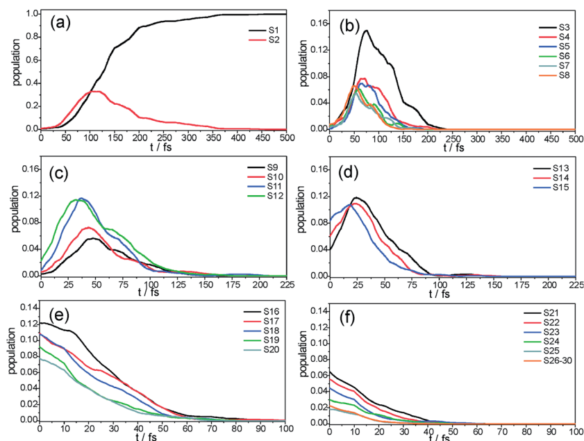
Fig. 4 Population of each electronic surface as a function of time obtained from the fraction of trajectories in each state.
