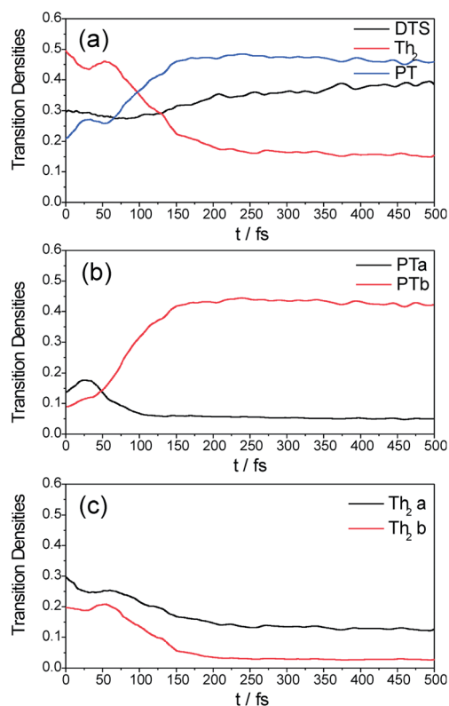
Fig. 6 Time-dependent average of the fraction of the transition density localized at the different units of the p -DTS(PTTh 2 ) 2 : (a) DTS, Th 2 , and PT, (b) PTa and PTb, and (c) Th 2 a and Th 2 b.
