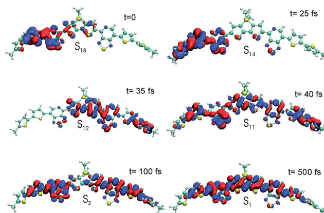
Fig. 7 Localization of the electronic transition density at different times along the representative trajectory in the NA-ESMD simulations.
