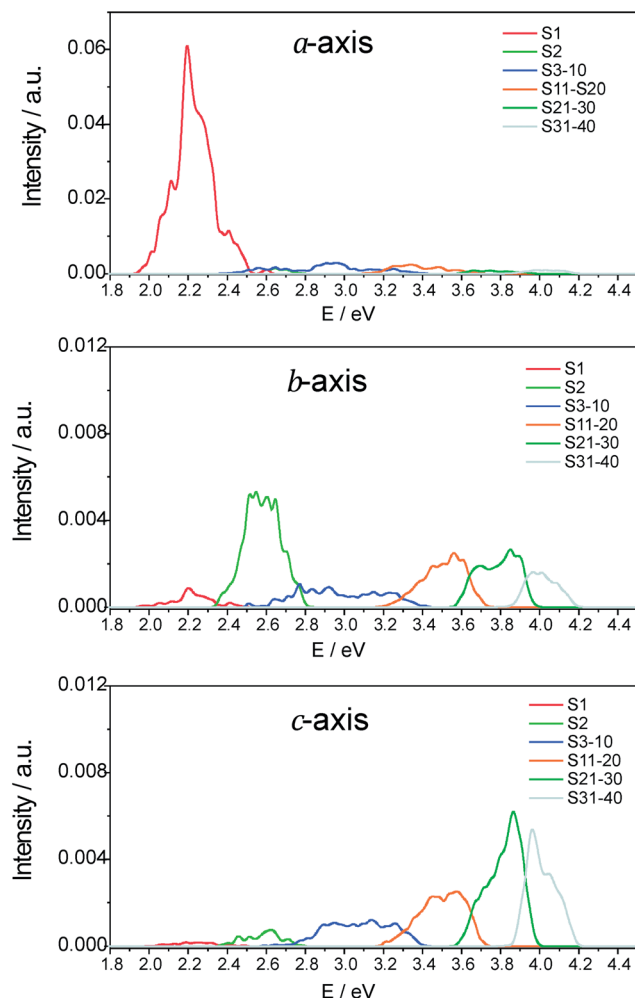
Fig. 2 (a–c) Relative absorbance intensities in the directions parallel to the a -, b - and c -inertial axes of the p -DTS(PTTh 2 ) 2 molecule.
