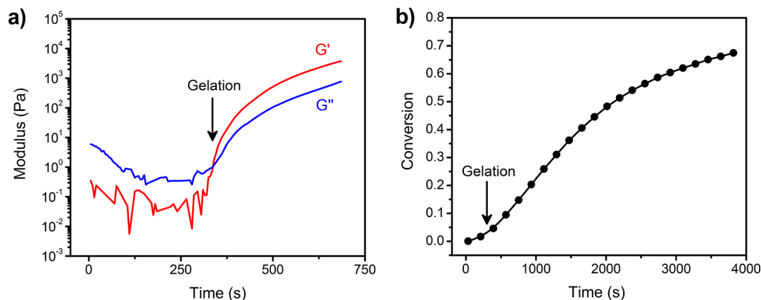
Figure 4. (a) Storage modulus ( G' ) and loss modulus ( G'' ) as a function of reaction time for a neat DGEBA sample cured by thermal cationic polymerization at 140 °C with \text{BF}_3 \cdot \text{MEA} as the initiator. (b) Real-time conversion profile for a neat DGEBA sample polymerized under the same reaction conditions as those used for the rheological experiment shown in (a).
