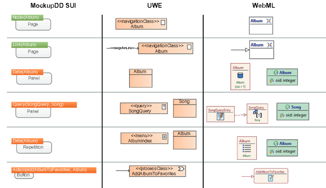
Fig. 8. Mapping from tagged SUIs elements to MDWE concepts.
