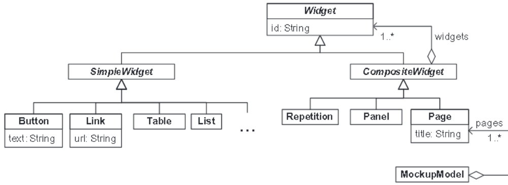
(a) Core SUI metamodel
