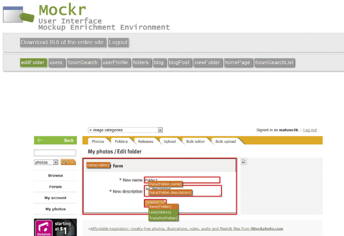
Fig. 11. Screenshot of the Interactive Tagging Tool.
