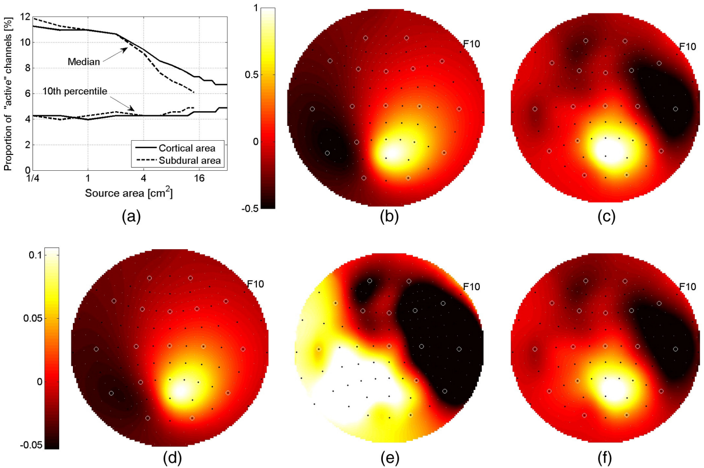
Fig. 3. (a) Proportion of channels with absolute amplitude greater than half the maximum. Median and 10th percentile of 1000 cortical generators for each generator area. (b) Normalized electric potential distribution of a generator with subdural extent 10 cm 2 . (c) Idem b with additive noise (SNR = 3). (d) Electric potential distribution of a generator with subdural extent 1.1 cm 2 . (e) The same as d with the same absolute noise level as c. (f) The same as d with the same relative noise level as c (SNR = 3).
