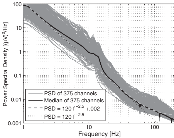
Fig. 4. A power spectral density (PSD) of 375 scalp EEG channels during non-REM sleep (gray), median (black full line), and approximations: background brain activity (dotted black line), and background brain activity plus electronic noise (dashed gray line).
