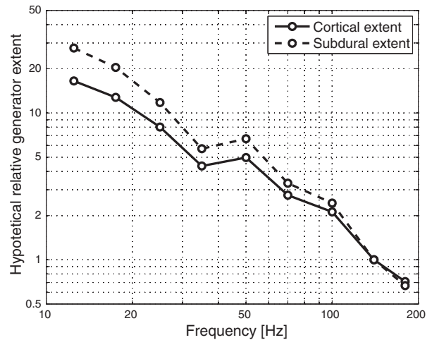
Fig. 6. Hypothetical median generator extent of the strongest interictal events as a function of frequency, relative to the median generator extent of the 120–160 Hz frequency band.
