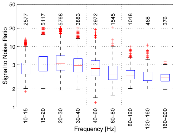
Fig. 5. Signal to Noise Ratio distribution of interictal epileptic events in different frequency bands. Median (red line), 25th and 75th percentiles (blue box), outliers (red crosses), and number of events in the frequency band (above).
