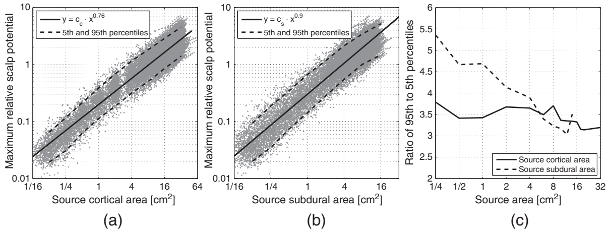
Fig. 2. Relationship between extent of the cortical generators and electric potential amplitude on the scalp. (a) Scatter plot of the maximum absolute scalp amplitude versus cortical extent of the generators (20,000 different generators as gray dots). The 5th and 95th percentiles are shown as dashed lines, and a power law fit with an exponent of 0.76 as a solid line. The amplitude is shown relative to the median value of generators of 10 cm 2 extent. (b) Idem a, but showing the results as a function of the subdural area of the generators. In this case the exponent of the power law is 0.9. (c) Relative variability of the general behavior shown as the ratio between the 95th and 5th percentiles as a function of the generator extent.
