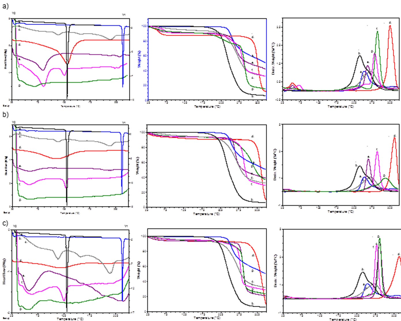
Fig. 5. DSC, TG and DTG curves of: (a) SMR:βCD:MEG; (b) SMR:MβCD:MEG and (c) SMR:HPβCD:MEG complexes. a. Pure SMR: blue; b. Pure MEG: black; c. Binary freeze-dried systems (BFDS) with MEG: gray; d. Pure CD: red; e. BFDS with the CD: purple; f. Ternary physical mixtures (TPM): pink; g. Ternary freeze-dried systems (TFDS): green; Scales: Y1 for SMR and MEG; Y2 for the remaining curves. (For interpretation of the references to color in this legend, the reader is referred to the web version of the article.)
