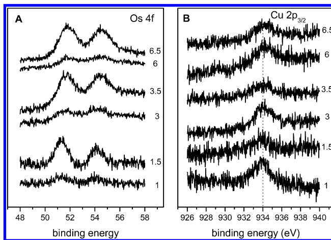
Figure 4. Os 4f (A) and Cu 2p 3/2 (B) XPS spectra of (PAH-Os/laccase) n self-assembled multilayers. Integer n represent laccase-terminated layers whereas fractional n represents Os-terminated layers.
