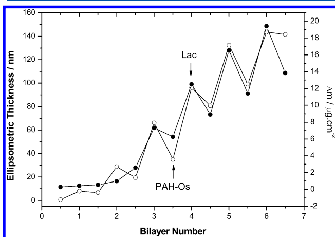
Figure 2. Ellipsometric thickness (open circles) and EQCM mass variation per unit area (solid circles), as a function of number of bilayers for different PAHOs/Laccase multilayers. The arrows indicate the macromolecule in the last layer.
