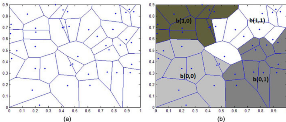
Figure 2. Spatial block bootstrapping. (a) Original sample. (b) Non-overlapping blocks.
